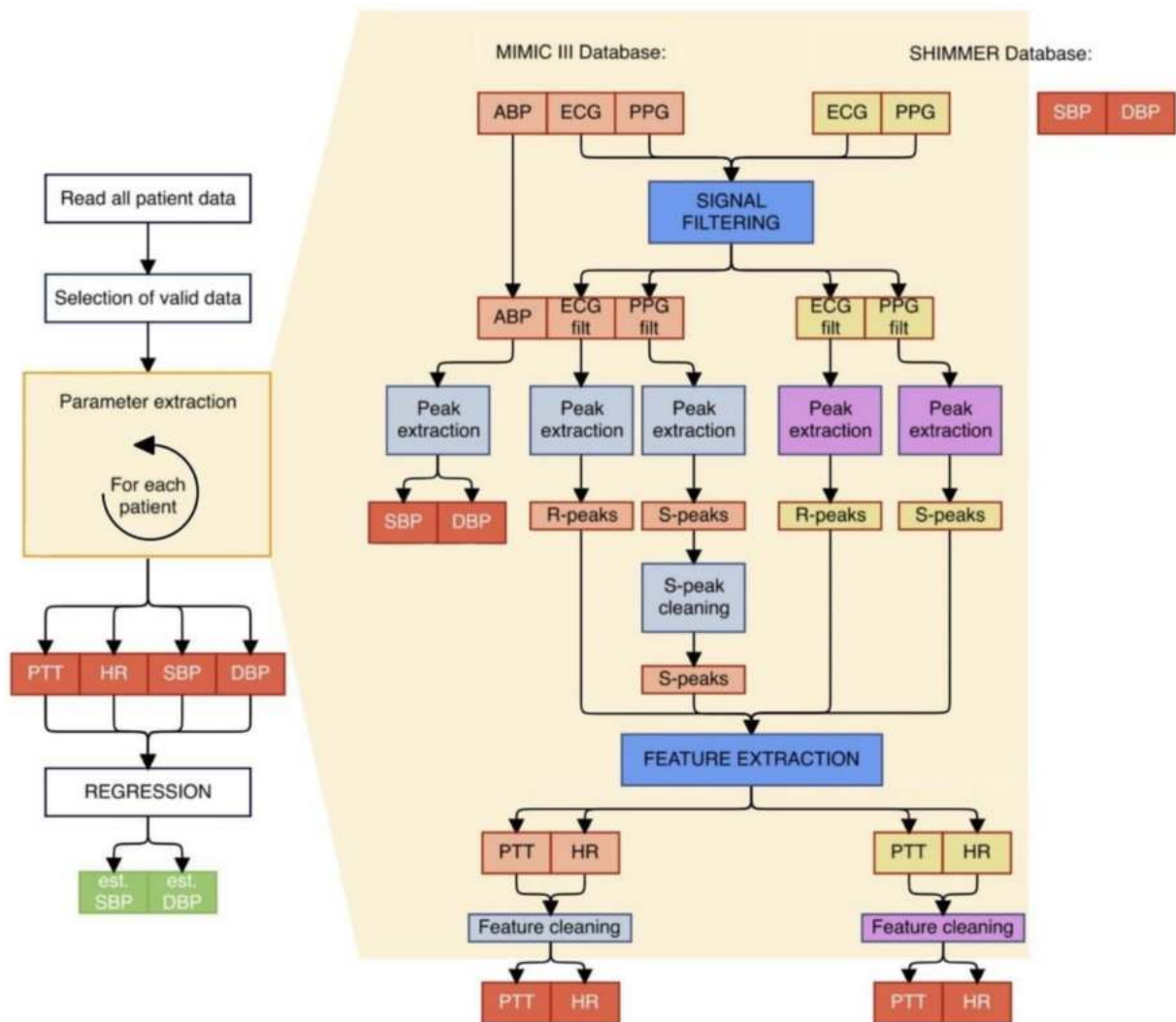
Figure 15. Algorithm structure.
