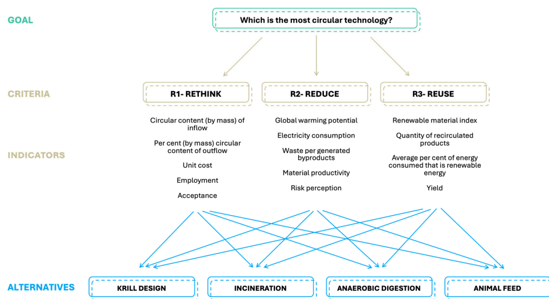
Figure 11. The hierarchy structure in the AHP.
