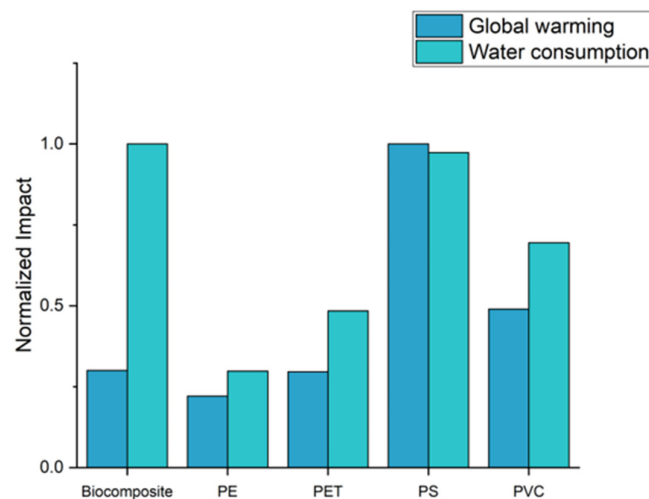
Figure 10. Normalized comparison of GWP and WC for biocomposite with traditional fossil-based polymers. PET: polyethylene terephthalate; PE: polyethylene; PVC: polyvinyl chloride; PS: polystyrene.
