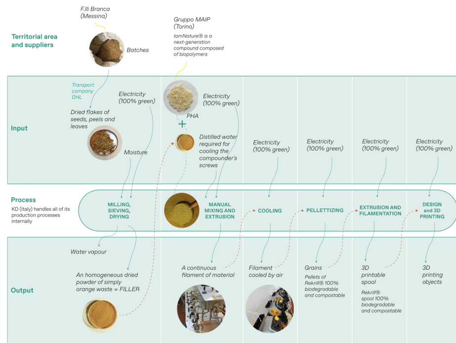
Figure 2. Descriptive scheme of the production process of Krill Design (KD), from cradle to gate. Solid arrows indicate input and output flows associated with each production stage, while dashed arrows indicate how the output of one stage serves as input for the subsequent stage. The green-shaded areas identify the inputs, processes, and outputs included in the production system.
