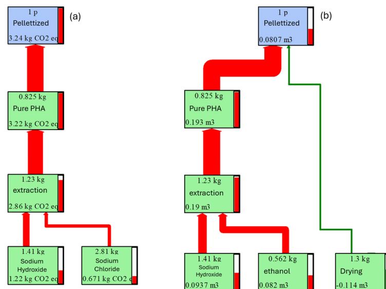
Figure 9. Sankey diagrams for GWP (cut-off of 15%) and WC (cut-off of 15%) to produce 1 kg of pelletized biocomposite (25% OPW, 75% PHA): (a) global warming potential (GWP, kg CO 2 eq); (b) water consumption (WC, m 3 ). Arrow width is proportional to the impact contribution: red indicates impacts generated, while green indicates impacts saved.
