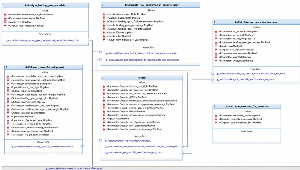
Fig. 3 Internal Block Definition Diagram of the landing gear subsystem highlighting mass and impact propagation
