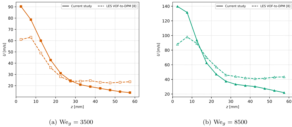
Fig. 10. Particles velocity magnitude downstream location for TC2 test cases.
