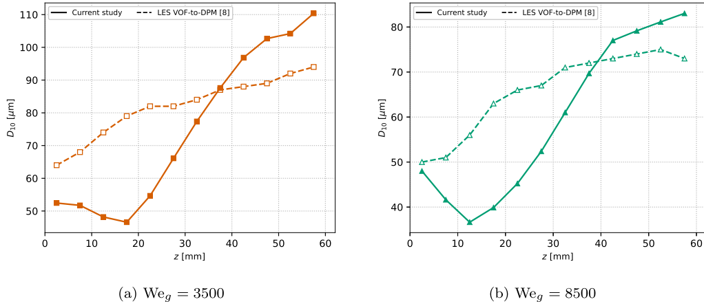
Fig. 9. D_{10} at x = 60 mm downstream location for TC2 test cases.
