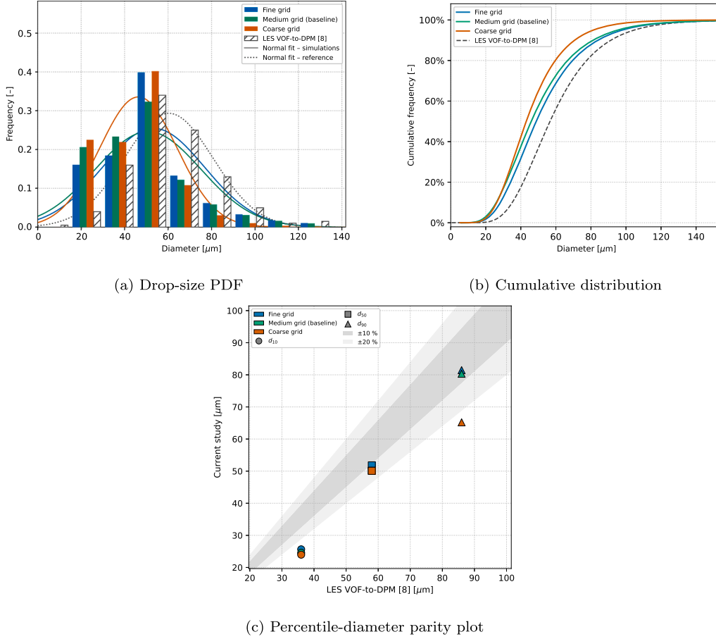
Fig. 2. Grid convergence at We_g = 8500 : (a) drop-size probability density function, (b) cumulative distribution, and (c) parity of the percentile diameters, for the coarse, medium (baseline) and fine grids compared with the LES VOF-to-DPM reference.
