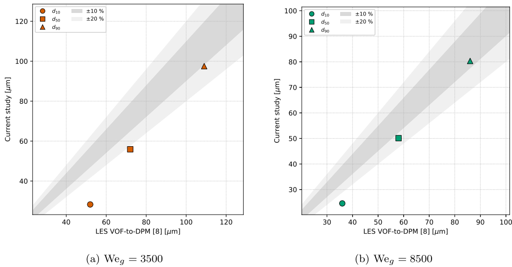
Fig. 13. Parity plots of d_{10} , d_{50} and d_{90} at x = 60 mm for TC2 test cases.
