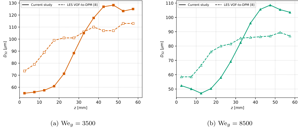
Fig. 8. D_{32} at x = 60 mm downstream location for TC2 test cases.
