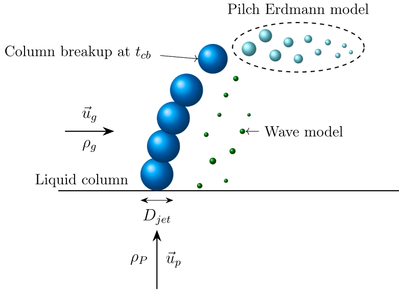
Fig. 1. Schematic representation of the Madabhushi breakup model. Adapted from Fluent manual [18].
