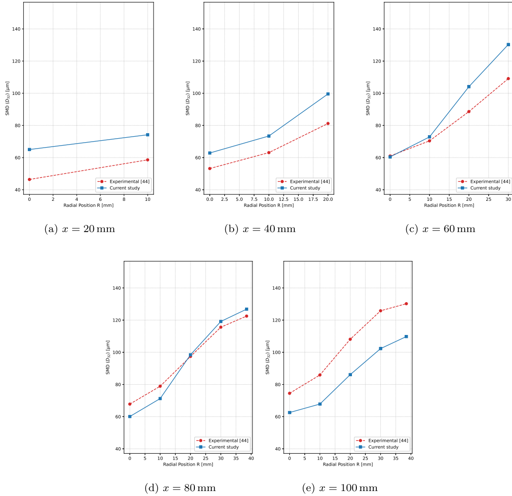
Fig. 5. SMD results at various downstream ( x ) and radial ( R ) locations for TC1-P1 test case.
