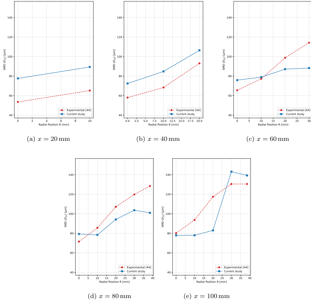
Fig. 6. SMD results at various downstream ( x ) and radial ( R ) locations for TC1-P2 test case.
