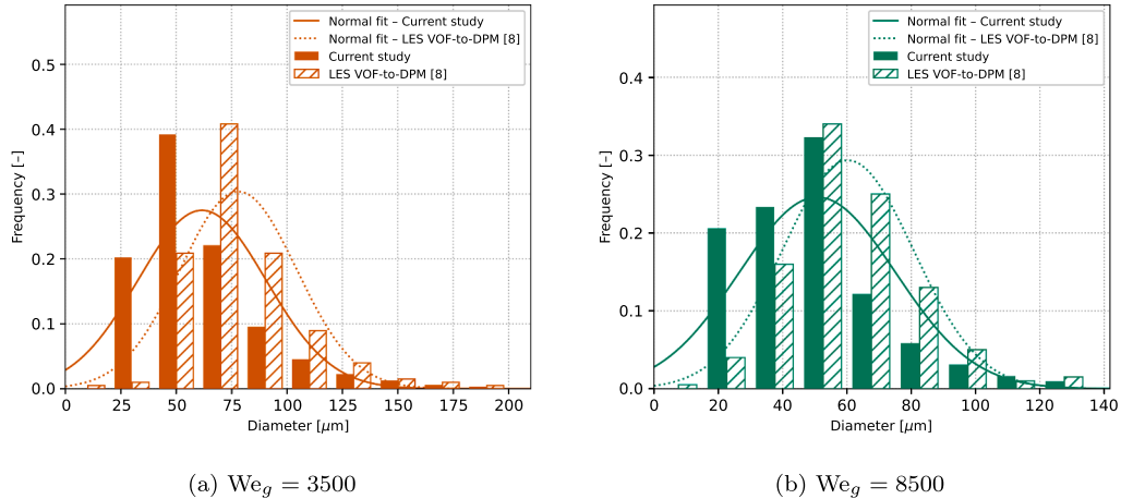
Fig. 11. Probability density function at x = 60 mm downstream location for TC2 test cases.
