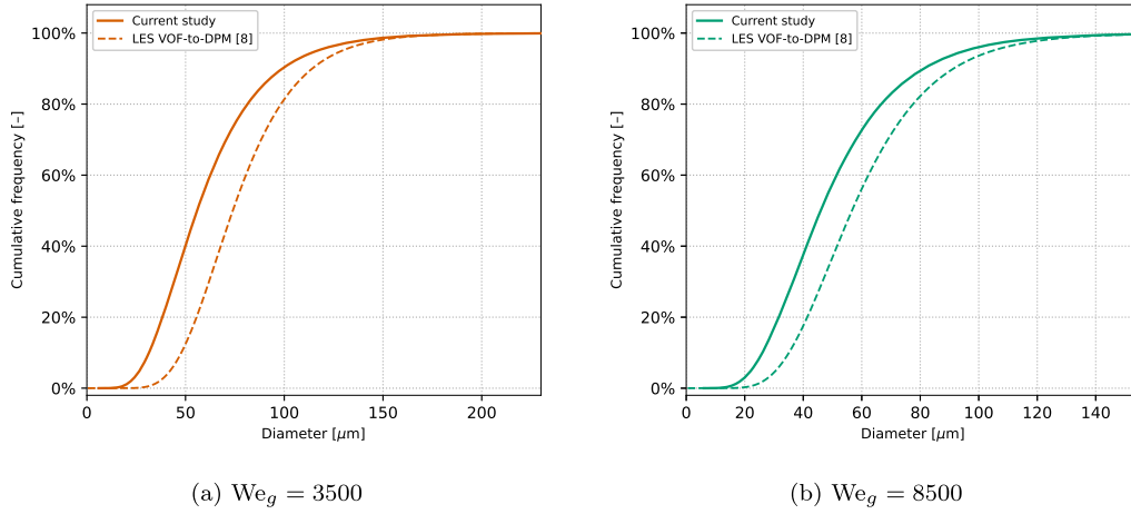
Fig. 12. Cumulative function at x = 60 mm downstream location for TC2 test cases.
