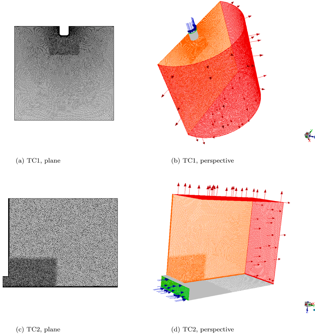
Fig. 4. Computational domains with mesh for TC1 and TC2 test cases.
