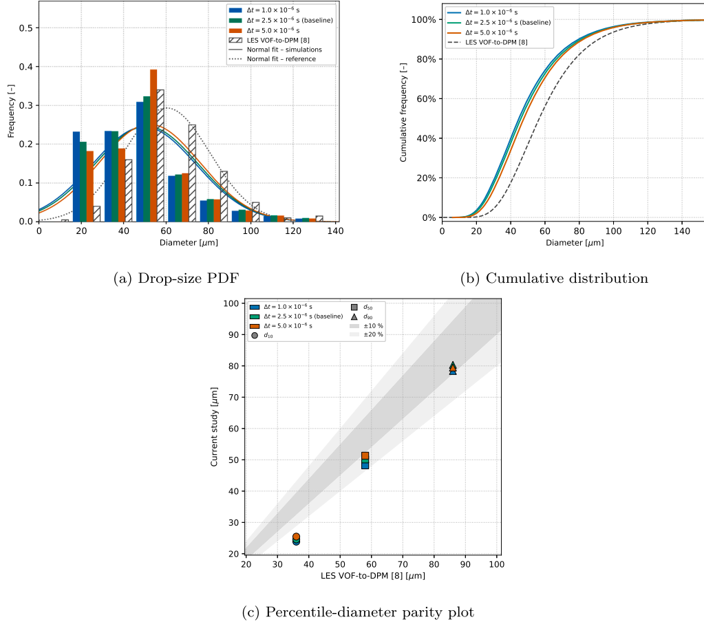
Fig. 3. Time-step convergence at We_g = 8500 : (a) drop-size probability density function, (b) cumulative distribution, and (c) parity of the percentile diameters, for \Delta t = 1.0, 2.5 (baseline) and 5.0 \times 10^{-6} s compared with the LES VOF-to-DPM reference.
