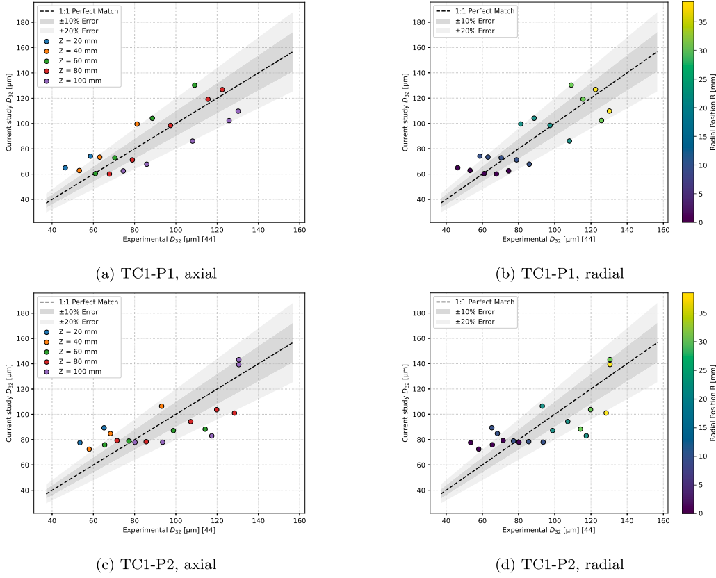
Fig. 7. Parity plot of SMD results for TC1 test cases.
