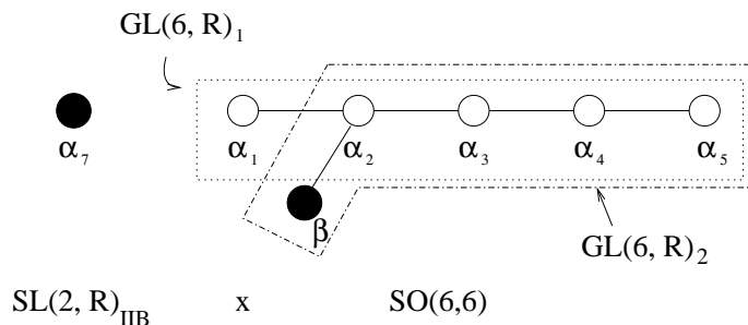
Figure 2: SL(2, \mathbb{R}) \times SO(6, 6)_T and SL(2, \mathbb{R}) \times SO(6, 6) Dynkin diagrams. The root \alpha is the E_{7(7)} highest root while \beta is \alpha_3 + 2\alpha_4 + \alpha_5 + 2\alpha_6 + \alpha_7 . The group SL(2, \mathbb{R})_{IIB} is the symmetry group of the ten dimensional type-IIB theory.
