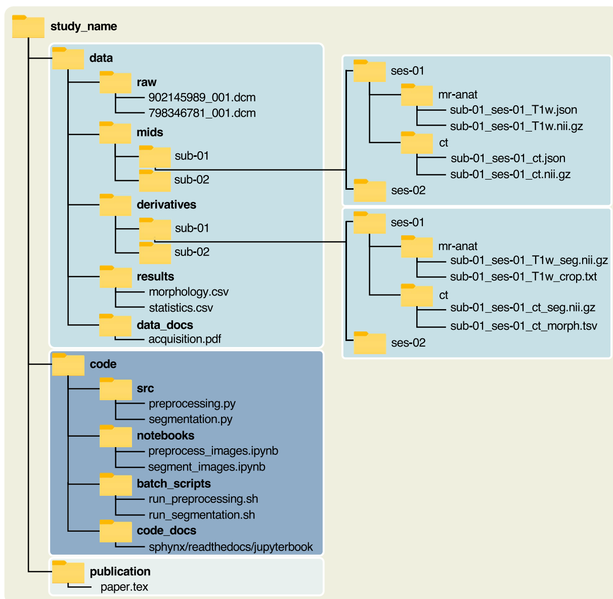
Figure 3 Folder and file structure of a computational research study for an open and reproducible publication. File extensions with acronyms expansions: .dcm: Digital Imaging and Communications in Medicine (standard file format for medical imaging data and associated metadata); .json: JavaScript Object Notation; .nii.gz: Neuroimaging Informatics Technology Initiative (compressed file format used to store medical imaging volumes); .txt: Plain Text; .tsv: Tab-Separated Values; .csv: Comma-Separated Values; .pdf: Portable Document Format; .py: Python Script; .ipynb: Interactive Python Notebook; .sh: Shell Script (script file containing commands for a Unix/Linux shell); and .tex: TeX (source file for documents written using the LaTeX typesetting system).
