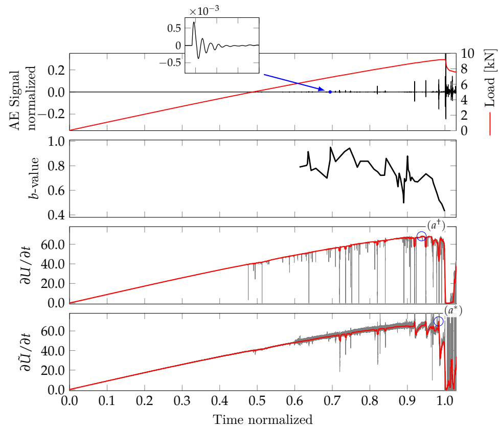
Figure 10. Results in terms of Acoustic Emission signal vs. time, load vs. time, and the time evolution of b -value and DPH index vs. the normalized time. Two measures of the DPH parameter are indicated: \partial U / \partial t indicate the derivative of the elastic energy computed internally in the simulation; \partial \tilde{U} / \partial t indicate the derivative of the measure of the elastic energy computed as the product between the reaction support and the prescribed displacement. (a^\dagger) and (a^*) instants of particular interest for the DPH computed using \partial U / \partial t and \partial \tilde{U} / \partial t .
