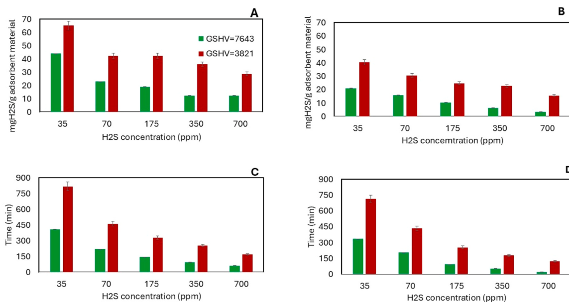
Fig. 3. A) and B) represent the adsorption capacity of CAC and KOH_RH_CO2, respectively, at gas space hourly velocity (GSHV) of 7643 (green) and 3821 h -1 (red). C) and D) represent the breakthrough time of CAC and KOH_RH_CO2, respectively.
