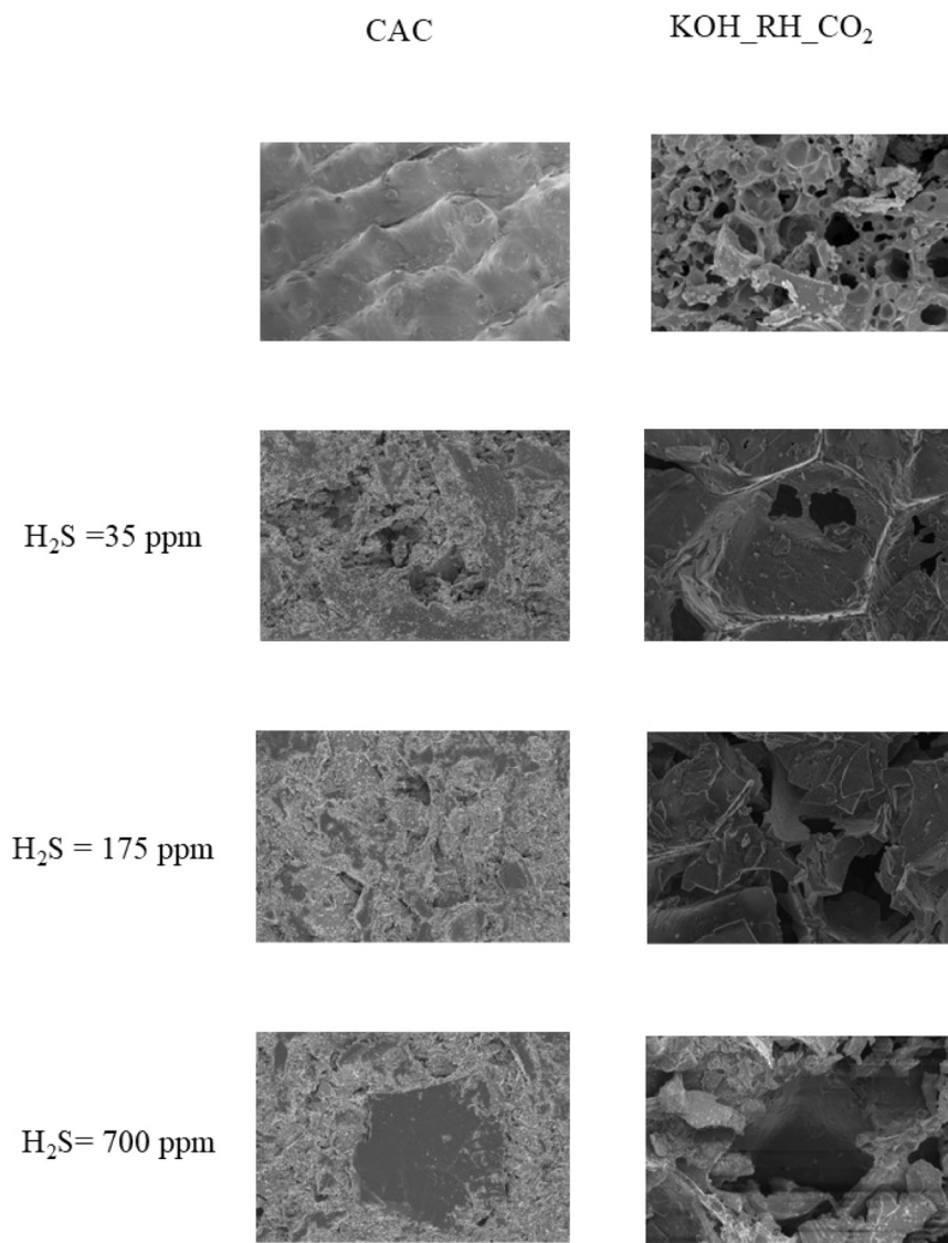
Fig. 5. FESEM analysis on CAC and KOH_RH_CO 2 at GHSV of 3822 h -1 with H 2 S concentrations of 35, 175, and 700 ppm. 2 \mu m scale with 5.00 KX magnification.
