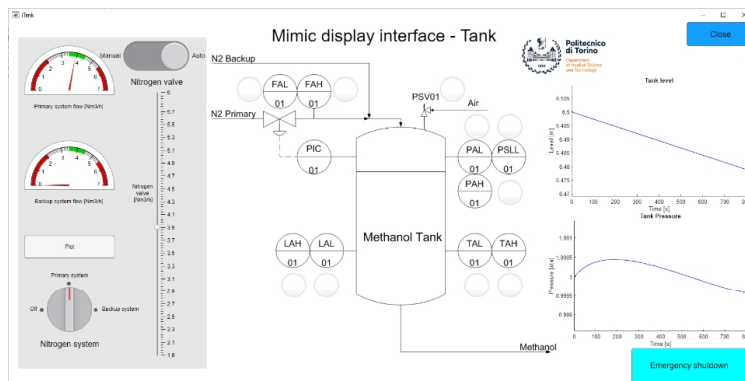
Fig. 4. Tank mimic (top left the close button; bottom down, the emergency button).
