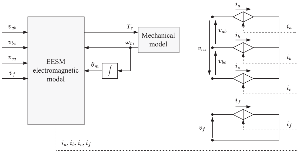
FIGURE 11. Proposed current-controlled generators model for EESMs.
