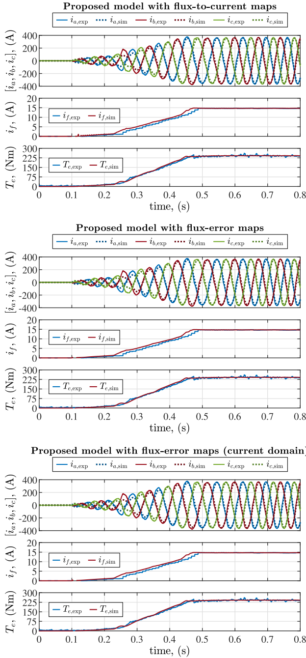
FIGURE 28. Torque transient test results for the proposed formulations of the decoupled-dynamics EESM model.
