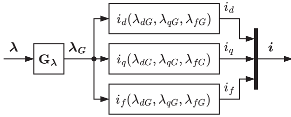
FIGURE 9. Currents determination in the single-step flux-based model [52].
