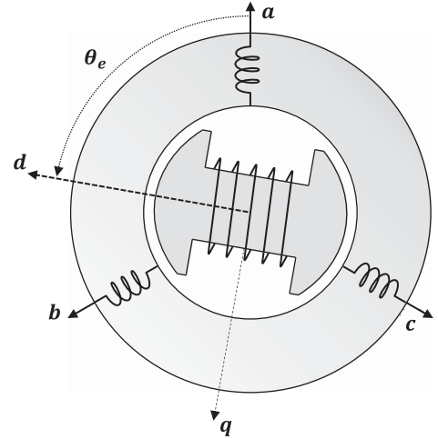
FIGURE 2. Schematic representation of a 2-pole EESM.
