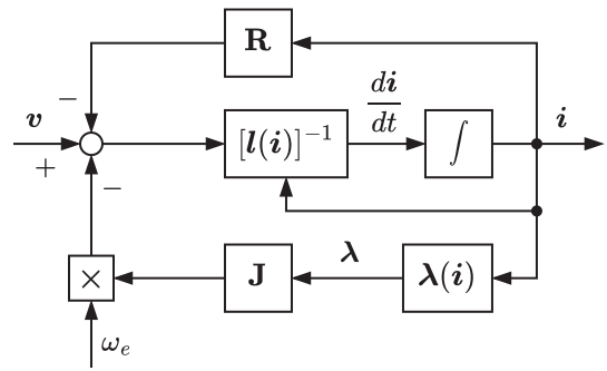
FIGURE 5. EESM current-based CCG model [50].
