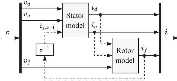
FIGURE 10. EESM model with decoupled dynamics.
