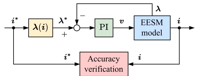
FIGURE 22. Block diagram for the accuracy verification of EESM models in simulation environment.
