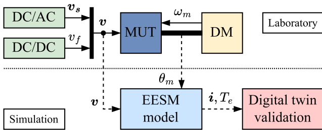
FIGURE 25. Block diagram of the digital twin tests for the experimental validation of EESM models.
