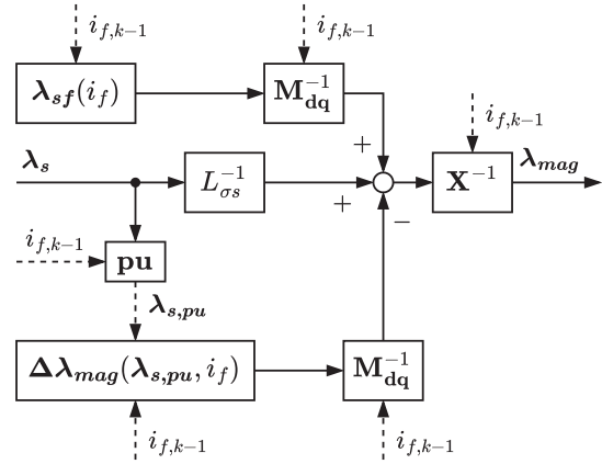
FIGURE 16. Computation of the stator magnetizing flux linkage.
