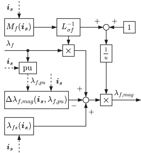
FIGURE 21. Computation of the rotor magnetizing flux linkage.
