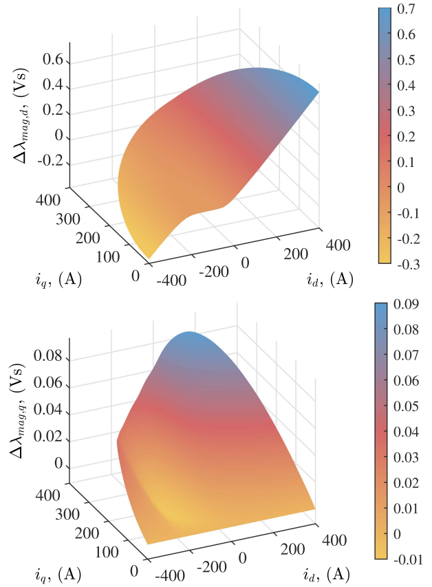
FIGURE 18. Stator flux-error maps with current domain of the EESM under consideration for i_f equal to 5 A.
