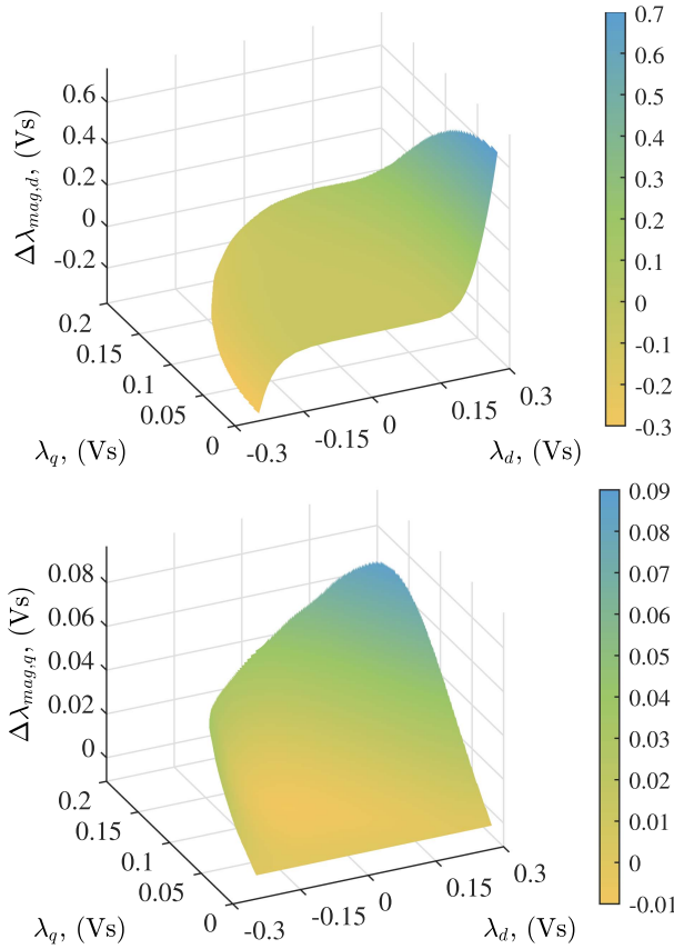
FIGURE 17. Stator flux-error maps of the EESM under consideration for i_f equal to 5 A.
