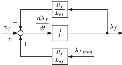
FIGURE 20. Rotor model for the approach with flux-error map [58].
