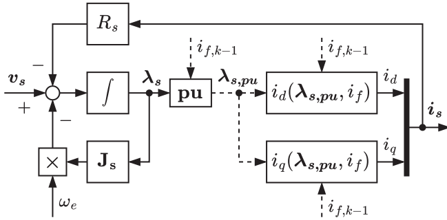
FIGURE 13. Stator model with flux-to-current maps [53].
