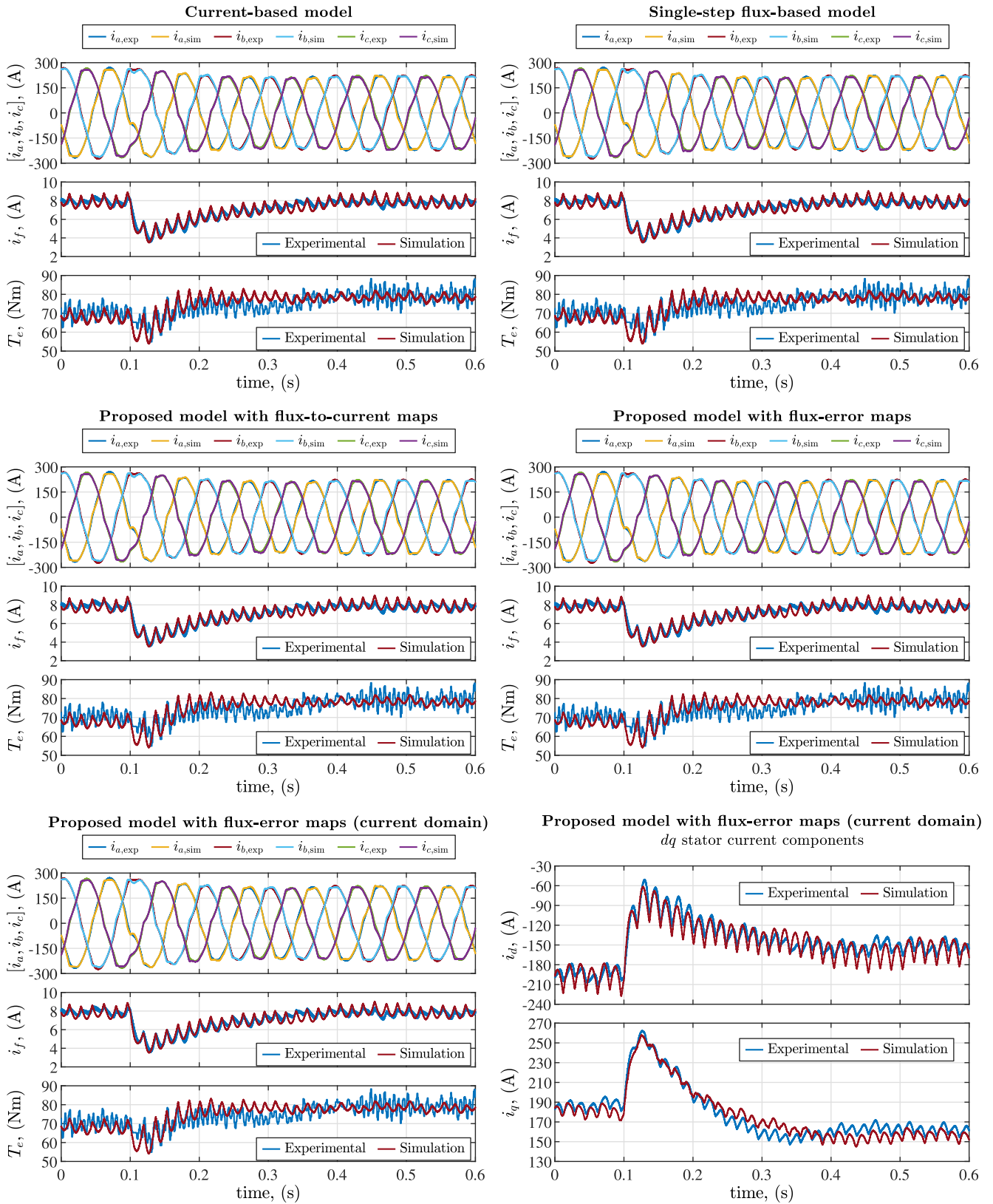
FIGURE 26. Results of the voltage steps test: comparison of experimental and simulation currents and torque for the state-of-the-art models and for the different formulations proposed for the EESM modeling with decoupled dynamics.
