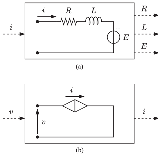
FIGURE 1. Circuitual representation of electric machine models. (a) voltage-behind-reactance – VBR. (b) current-controlled generators – CCG.
