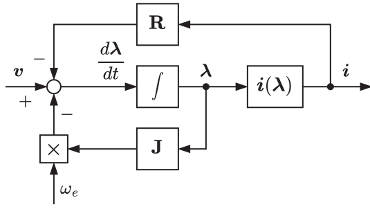
FIGURE 6. EESM single-step flux-based CCG model with flux-to-current maps [52].
