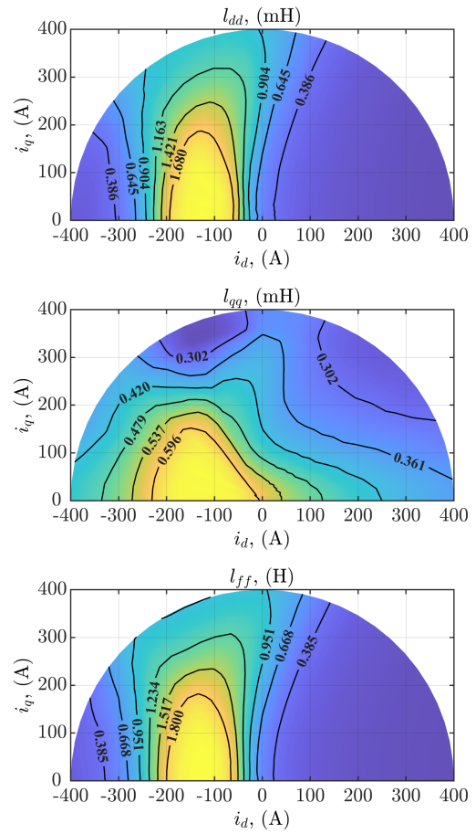
FIGURE 4. Incremental inductances of the EESM under consideration for i_f equal to 5 A.
