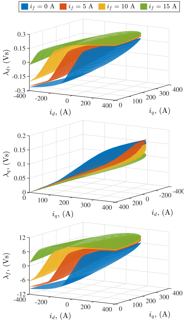
FIGURE 3. Current-to-flux maps of the EESM under consideration.
