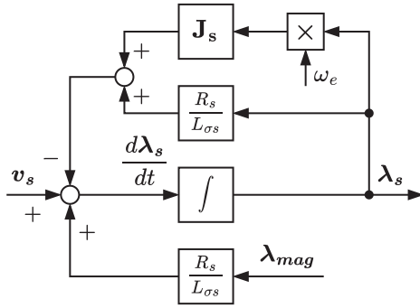
FIGURE 15. Stator model for the approach with flux-error maps.
