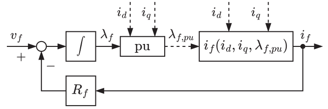
FIGURE 14. Rotor model with flux-to-current map.
