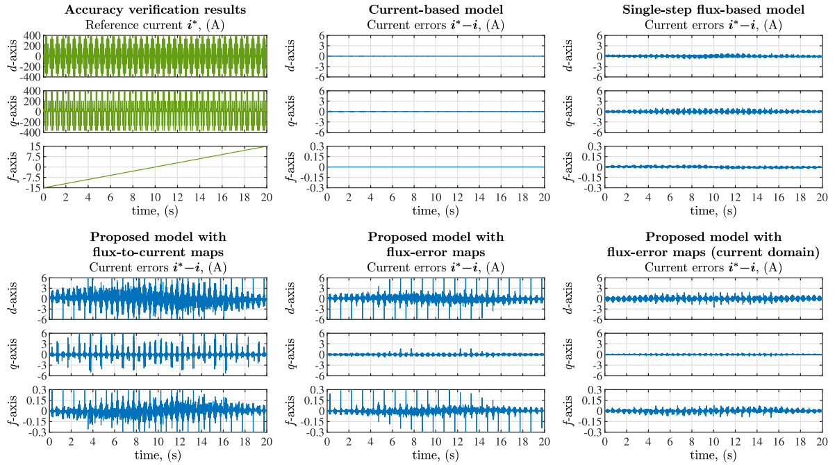
FIGURE 23. Reference current vector and results of the accuracy verification in simulation for the considered EESM CCG models.
