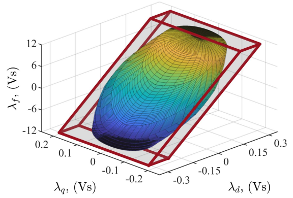
FIGURE 8. Improved domain selection for the flux-to-current maps.
