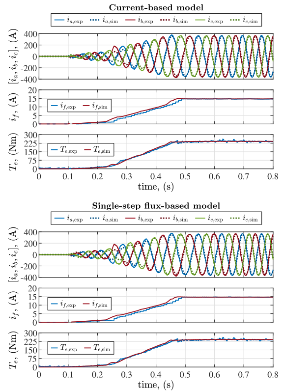
FIGURE 27. Results of the fast torque transient test for the state-of-the-art current-based and single-step flux-based models.
