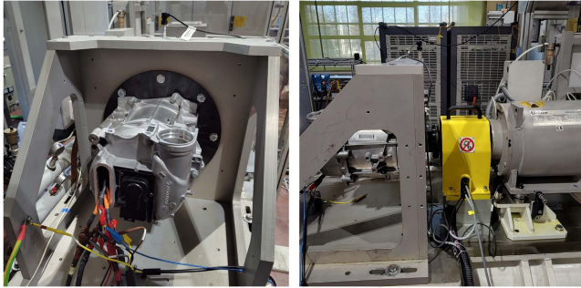
FIGURE 24. Test rig for the experimental validation: EESM under test (left), torque transducer (inside the yellow case) and driving machine (right).
