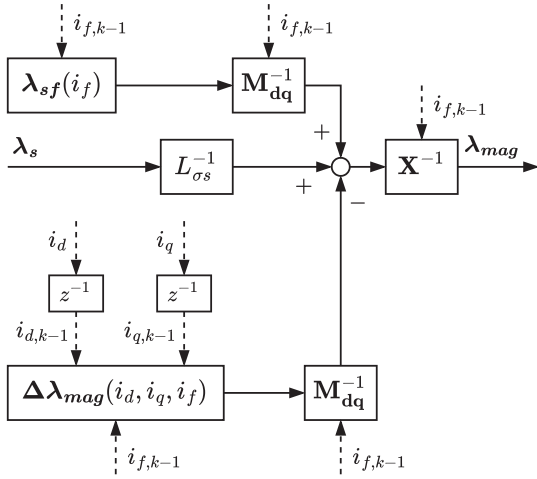
FIGURE 19. Computation of the stator magnetizing flux linkage by means of flux-error maps with current domain.
