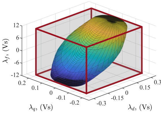
FIGURE 7. Flux linkages and the smallest external cuboid domain.
