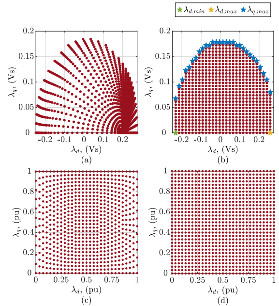
FIGURE 12. Elaboration of the stator flux-to-current maps domain for the EESM under consideration. (a) Stator flux linkages for i_f equal to 5 A. (b) Boundaries determination. (c) Normalized domain. (d) Final flux domain.
