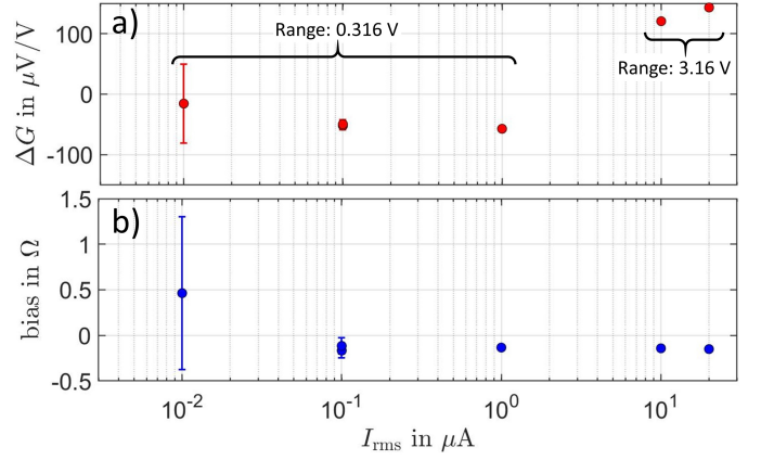
Figure 3. Current dependence of the gain error (a) and bias (b) of the bridge calculated from the QHE resistance measured at 22 Hz on the plateaus. The uncertainty bars correspond to the Type A uncertainties obtained over 10 measurements.
