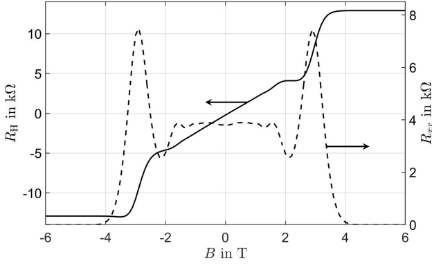
Figure 2. B dependency of R_H (solid line) and R_{xx} (dashed line) measured at 22 Hz and 100 nA on graphene device.
