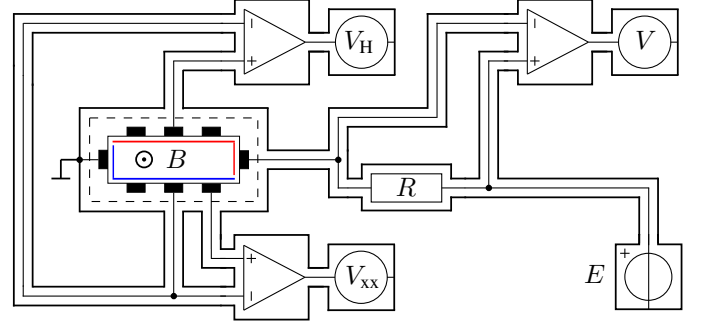
Figure 1. Bridge schematics designed for the characterization of the magneto-transport properties of the QAHE devices.
