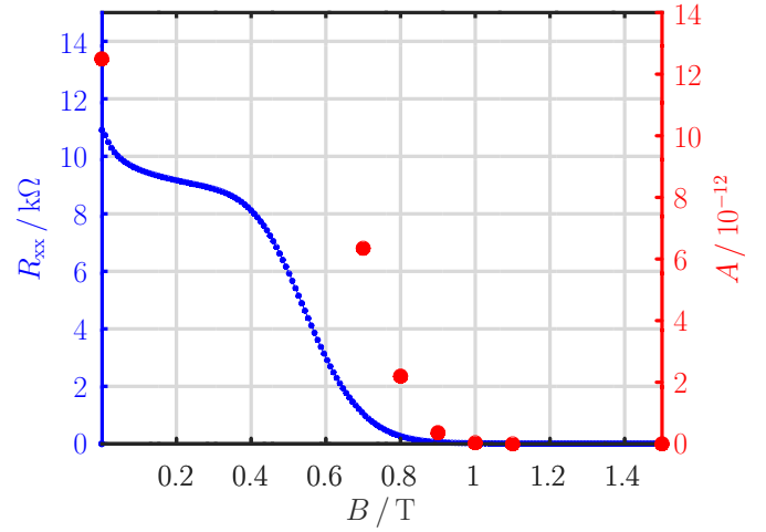
Fig. 3. (•) Flicker noise magnitude A_{V_H} and (•) longitudinal resistance R_{xx} versus the applied magnetic field B , see also Figure 2 and Sec. IV.
