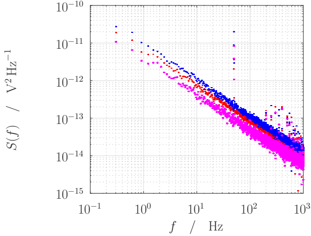
Fig. 2. An example of measurement outcome. Sample G52, B = 0.7 T, T = 3.6 K, I = 10 \mu A. (•) S_{V_H}(f) , (•) S_{V_{xx}}(f) , (•) S_{V_H, V_{xx}}(f) .
