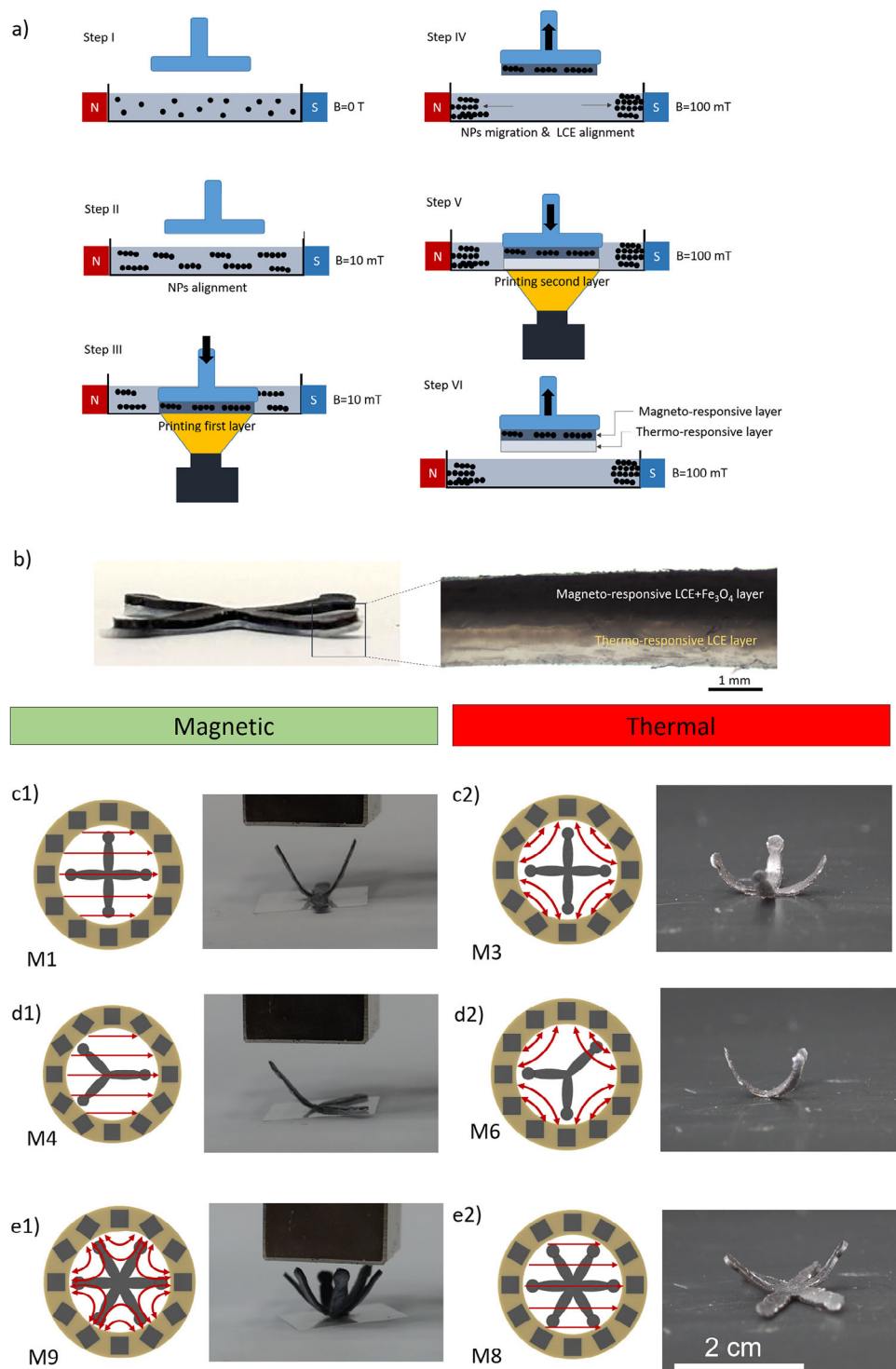
Figure 4. Multimodal thermo-magnetic actuation in composite LCEs embedding \text{Fe}_3\text{O}_4 nanoparticles. a) Schematic of the fabrication sequence for a thermo-magnetic bifunctional material. b) Cross-sectional optical image showing a bilayer structure composed of isotropic \text{Fe}_3\text{O}_4 nanoparticle chains within non-aligned LCE mesogens (dark color) and an aligned LCE layer (bright color). Distinct magnetic modes were encoded in three architectures: cross-shaped, Y-shaped, and hexapod. For the cross, (c1) shows magnetic mode M1 with two activated arms, while (c2) shows thermal mode M4 engaging all four arms. In the Y-structure, (d1) corresponds to magnetic mode M4 with one activated arm, and (d2) to thermal mode M6 activating all arms. For the hexapod, (e1) represents magnetic mode M9, where a hexapolar Halbach configuration drives coordinated activation of six arms, and (e2) thermal mode M8, inducing two bending and four twisting deformations.
