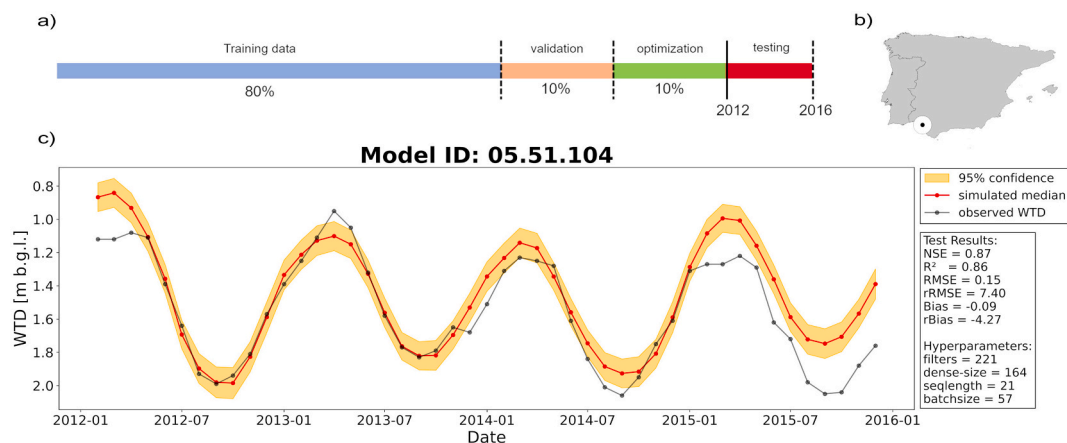
Fig. 2. a) Time series splitting scheme for training (80 %), validation (10 %), optimization (10 %), and testing (last four year) periods. b) Approximate location of the well in the region. c) Hyperparameters and model's performance using several statistical metrics for a random well (ID 05.51.104) during the test period [2012–2016].
