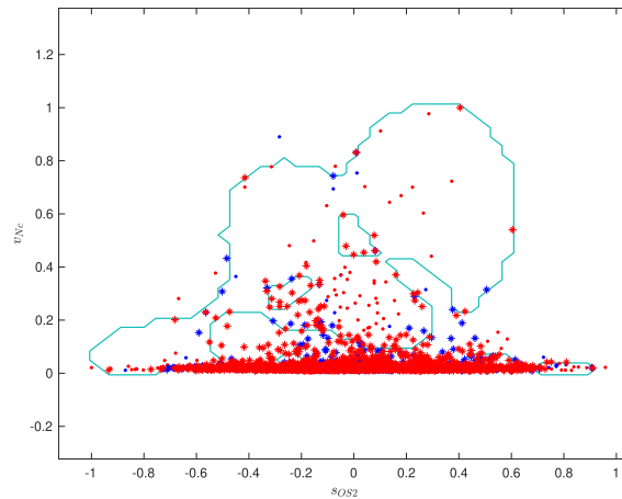
FIGURE 10. 2D graph of the “adversarial region” (the red points are the attacked ones) with s_{OS2} (Skewness of operational setting 2) and v_{Nc} (Variance of physical core speed) as input features of the CW-RUL dataset. The star points are the SVs of the description, coloured referring their specific label.
