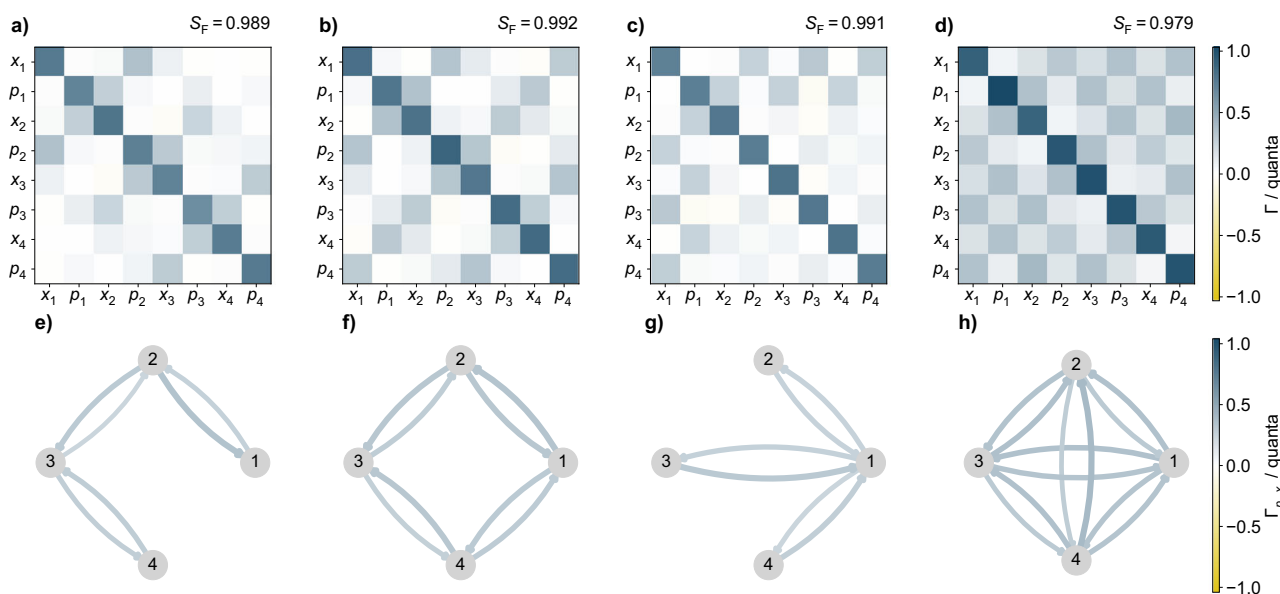
Fig. 3 | Quadrature covariance matrices and inferred graph connectivity. a–d Reconstructed covariance matrix \Gamma of the quadrature operators at P_p = -24 dBm, extracted from heterodyne detection of four frequency modes clustered in linear ( a , e ), cyclic ( b , f ), star ( c , g ), and fully-connected ( d , h )
