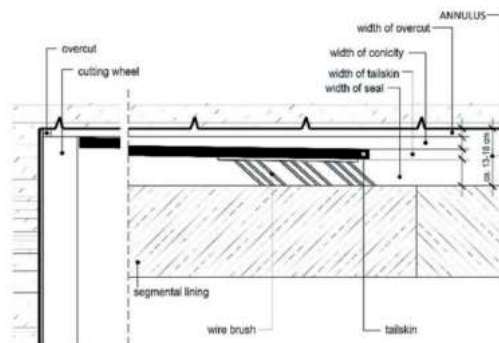
Figure 1. Annulus. Modified from thewes and budach (2009).
