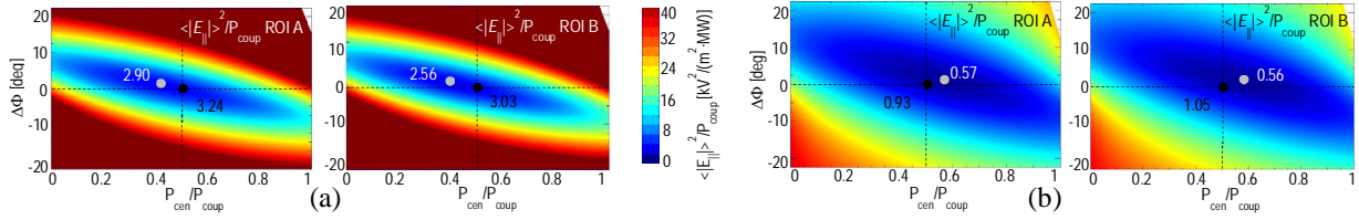
FIGURE 7. \langle |E_{||}|^2 \rangle / P_{\text{coup}} with [0; \pi; \pi; 0] , from TOPICA data: a) [0; -\pi/2] poloidal; b) and [0; \pi] poloidal.
