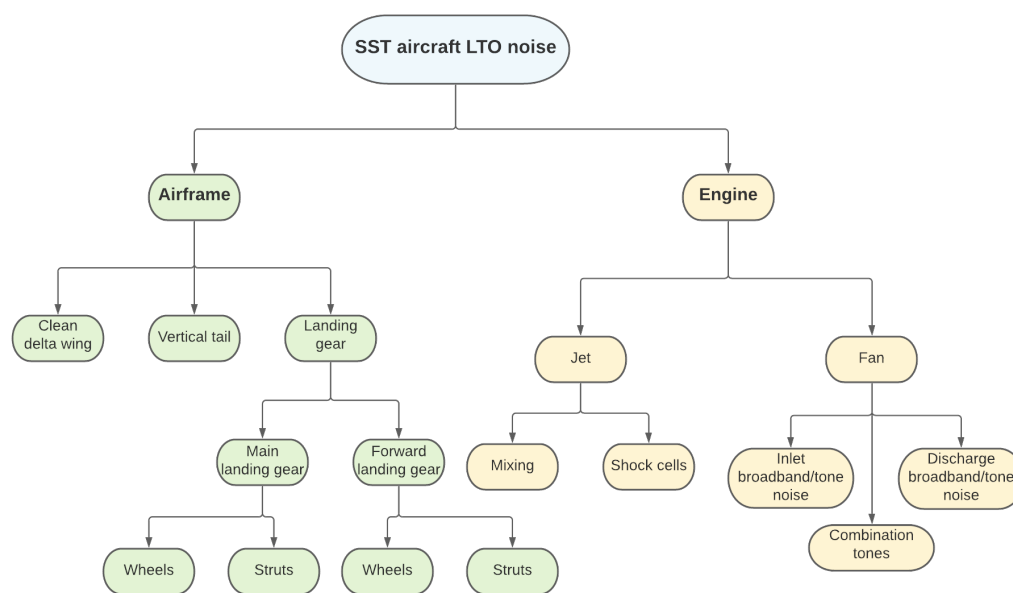
Figure 3. SST aircraft LTO noise sources break-down.
