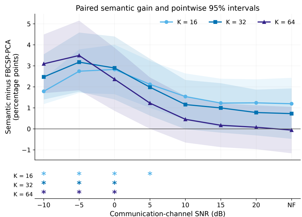
Figure 3. Semantic-minus-FBCSP–PCA balanced-accuracy difference. Bands show descriptive pointwise 95% confidence intervals; asterisks in the lower rows denote exact max- |t| -adjusted p < 0.05 ; NF, noise-free.
