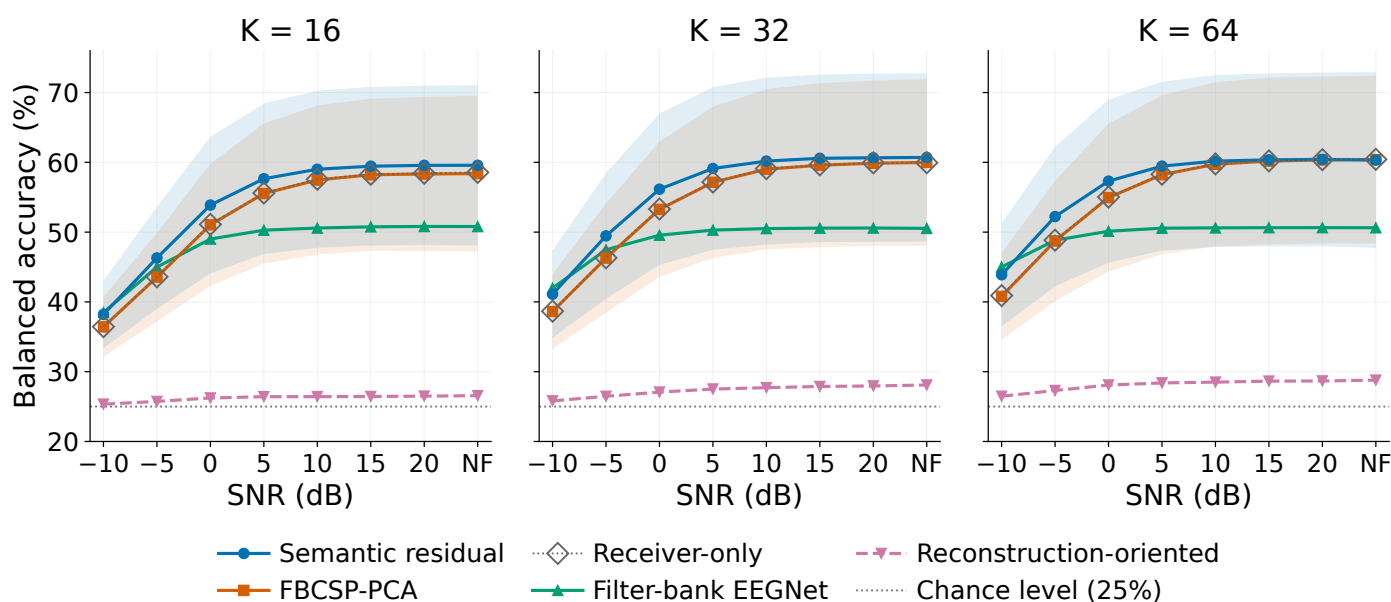
Figure 2. Balanced accuracy across message dimensions for all five comparison methods. Bands show descriptive 95% confidence intervals for the semantic and FBCSP-PCA means; NF, noise-free.
