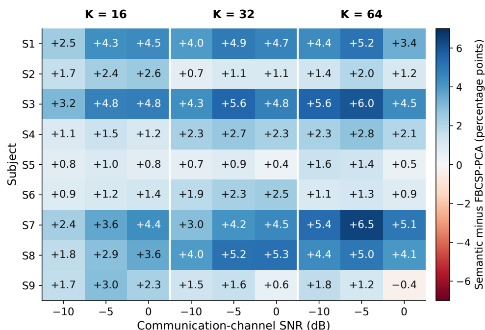
Figure 4. Subject-level semantic-minus-FBCSP-PCA balanced-accuracy differences at low SNR (percentage points).
