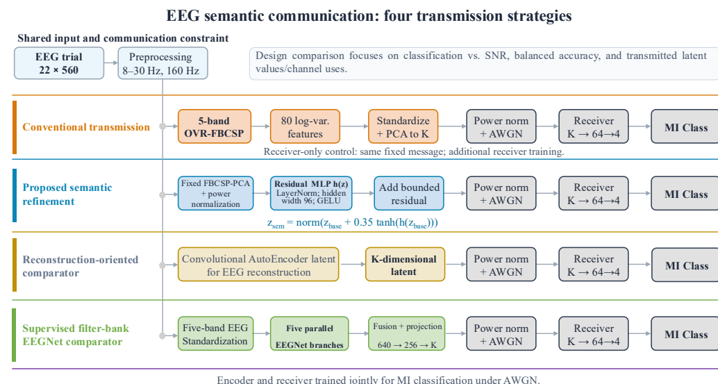
Figure 1. Remote MI-classification framework and four message representations. All methods transmit K power-normalized real values through AWGN; the receiver-only control retains the conventional message. OVR, one-versus-rest; MLP, multilayer perceptron; GELU, Gaussian error linear unit.
