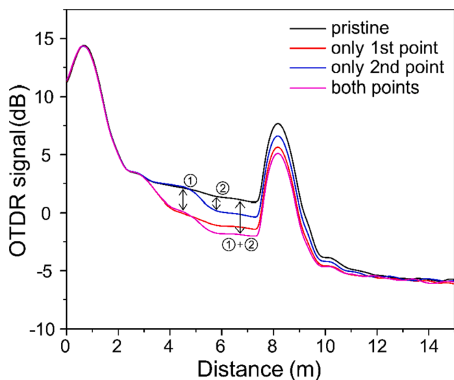
Fig. 10. Experimental demonstration of multiple leaks detection. The sensing fiber is exposed to dichloromethane at a first location ( \sim 3 m), and at a second location ( \sim 5 m), in two separate experiments. In a third test, the leakage is simulated at both locations, producing a double drop step in the OTDR trace. Therefore, the two leakage events appear detectable.
