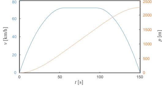
Fig. 1. Reference trajectory of the leading train.
