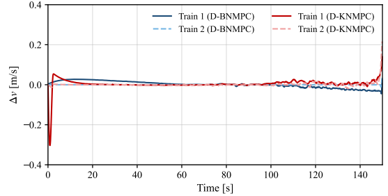
Fig. 3. Time [s] - speed deviation [m/s].
