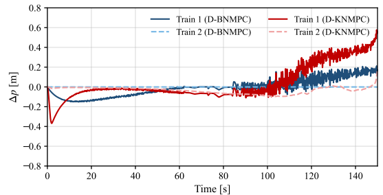
Fig. 4. Time [s] - spacing deviation [m].
