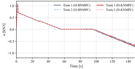
Fig. 5. Time [s] - Control force [kN/t].
