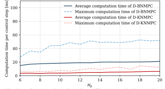
Fig. 2. Computation time for different predictive horizons
