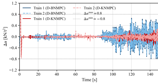
Fig. 6. Time [s] - change rate of control force [kN/t 2 ].
