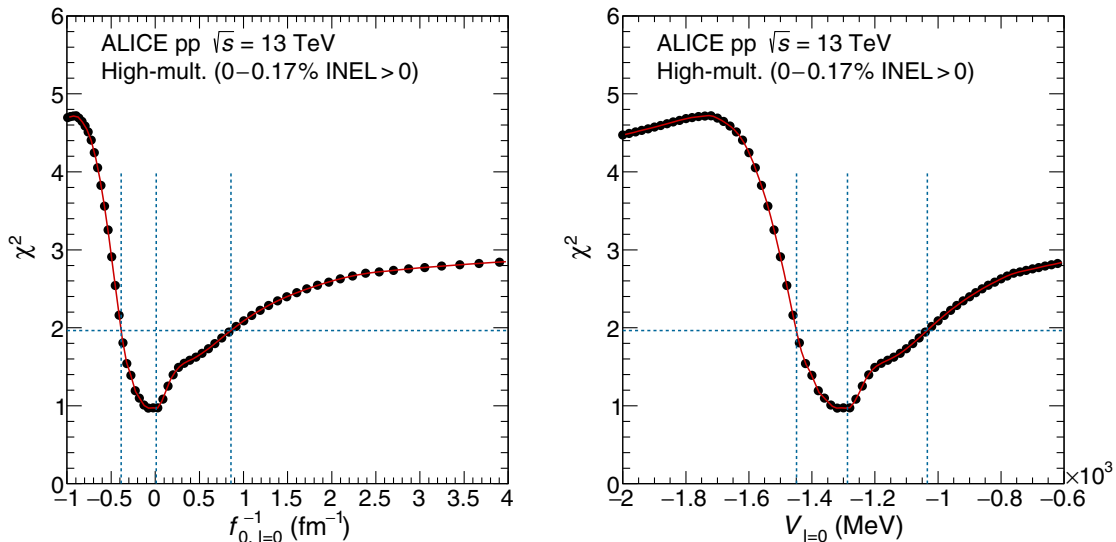
FIG. 4. \chi^2 distributions obtained by comparing the measured C_{pD^-}(k^*) for k^* < 200 MeV/c with the correlation function calculated with an interaction modeled by a Gaussian potential with an interaction range given by \rho -meson exchanges as a function of the inverse scattering length (left panel) and the interaction potential (right panel) for I = 0 . The blue dotted lines represent the value of f_{0,I=0}^{-1} and V_{I=0} = 0 for which the \chi^2 is minimum and for the 1\sigma confidence interval.
