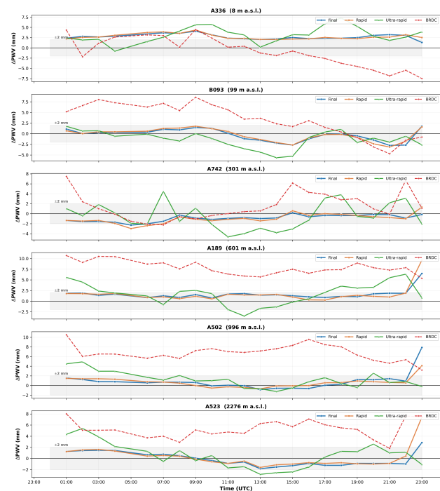
Figure 6. Hourly GNSS PWV – ERA5 TCWV difference time series for six representative stations. Grey shading indicates the \pm 2 mm band.
