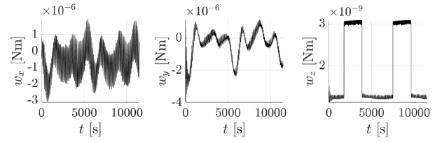
Fig. 1. Evolution over two orbital periods of the total torque due to the environmental disturbance sources.
