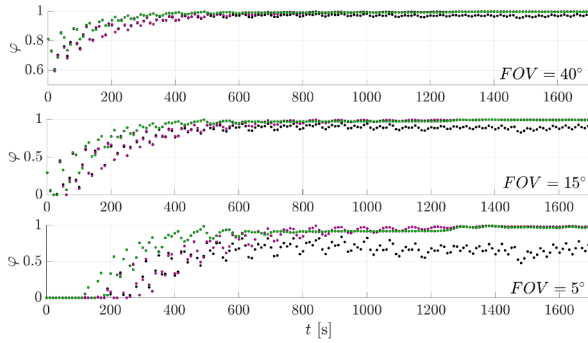
Fig. 8. Evolution of the relative misalignment between the projected area \mathcal{E}_{id} of the ideal cone and the one \mathcal{E}_R of the controlled cone when employing LQMP (black), TRMPC (magenta), and OS-SMPC (green). (For interpretation of the references to colour in this figure legend, the reader is referred to the web version of this article.)
