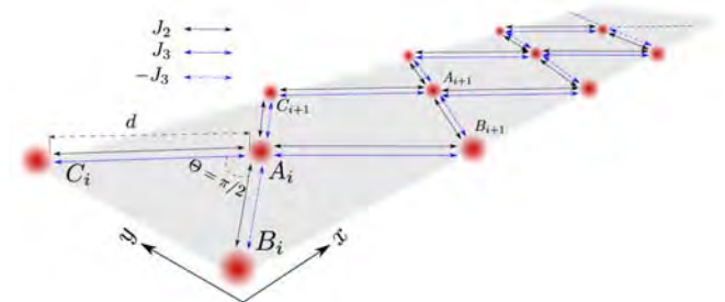
FIG. 71. Schematic representation of the considered diamond chain.
