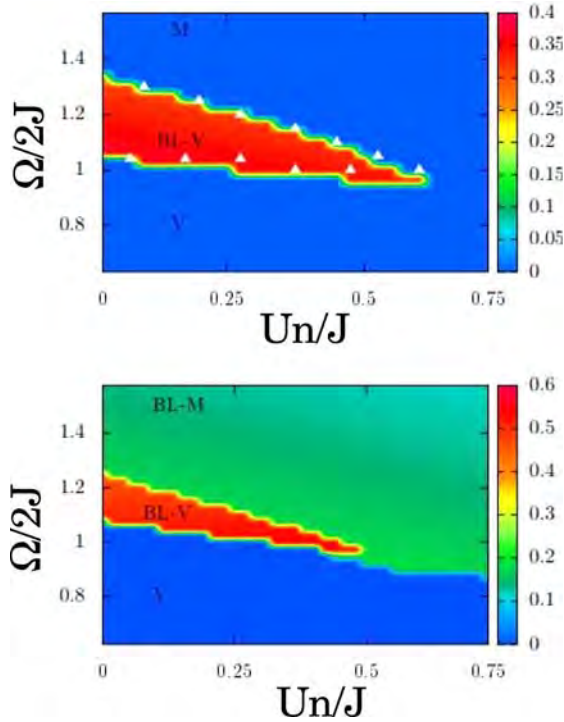
FIG. 67. Color map of the imbalance among particle numbers in each ring, in the (\Omega/J, U_{\perp}/JN_s) plane, for (upper panel) \lambda = \pi/2 , \Phi = 6\pi/N_s and N_s = 20 , (lower panel) \lambda = \pi/2 , \Phi = \pi/N_s and N_s = 20 . The letters indicate the parameter regimes where we find a biased-ladder phase (BL-V) where the single-particle spectrum has a double minimum, a Meissner phase (M), a vortex phase (V) and a biased-ladder phase (BL-M) where the single-particle spectrum has a single minimum. White triangles represent the frontiers between biased-ladder phase the two other phase, namely, vortex phase and Meissner phase as calculated with the variational ansatz including finite size effect.
