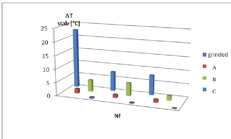
Fig. 6 \Delta T_{stab} vs cycles to failure. 10 Hz
