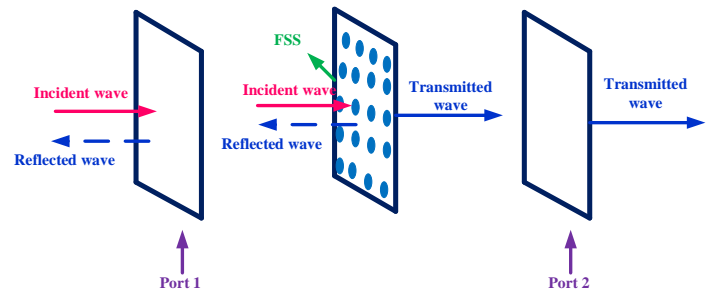
Fig. 1. Representation of different phenomena when an incident wave hits a FSS. Port 1 and port 2 correspond to the observation sections on the two sides of the FSS structure.
