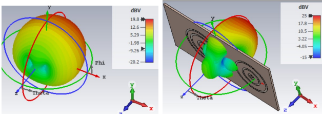
Fig. 8. Radiation pattern of the initial (left) and expanded (right) optimized FSS at 11 GHz.
