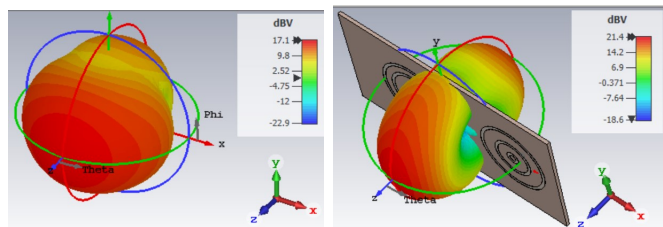
Fig. 7. Radiation pattern of the initial (left) and expanded (right) optimized FSS at 9.2 GHz.
