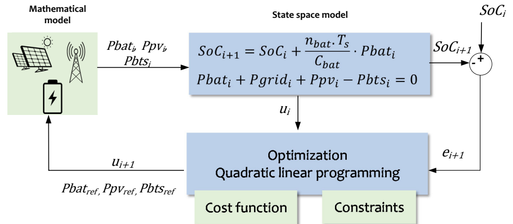
Figure 3. Block diagram of the Adaptive Model Predictive Control (AMPC) framework.
