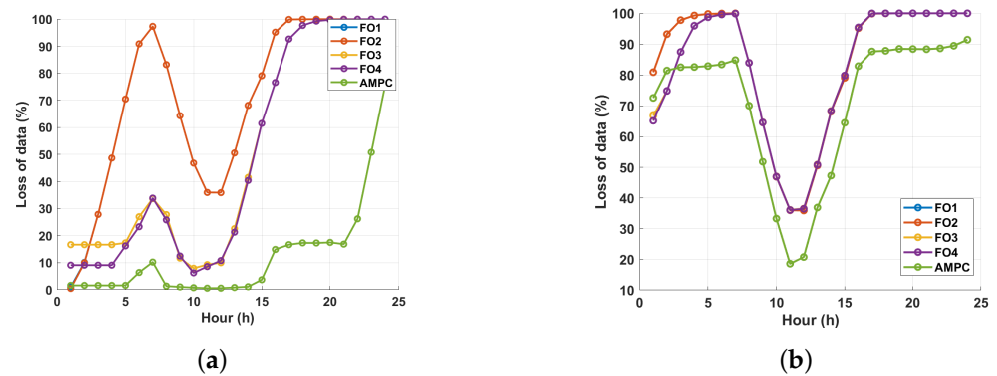
Figure 11. Comparison of BTS traffic data loss across all control strategies (FO 1 –FO 4 and AMPC) for two BESS SoC levels: (a) Percentage of loss of traffic data when BESS SoC is 50%. and (b) Percentage of loss of traffic data when BESS SoC is 20%. Data loss is estimated proportionally to power curtailment during grid outages.
