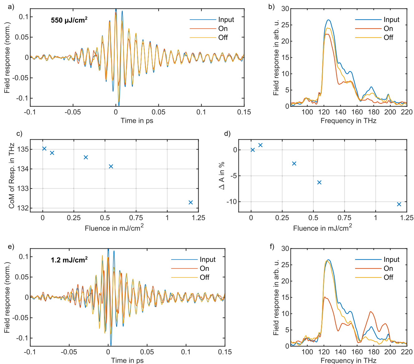
Figure 4. Reversible optical switching dynamics and fluence-dependent modulation in ITO. a) Reversibility response of the optical switching at the fluence of 550 \mu\text{J cm}^{-2} . The 'Input' trace shows the response field at low fluence. 'ON' corresponds to the response field at 550 \mu\text{J cm}^{-2} , while 'OFF' represents the response field measured at low fluence after switching. b) The spectral response of switching at the fluence of 550 \mu\text{J cm}^{-2} . c) Weighted mean frequency of the response at various fluences. A red shift in the weighted mean frequency is observed as the fluence increases up to 1.2 \text{ mJ cm}^{-2} . d) Modulation depth of the switch at various fluences. The integrated \Delta A is calculated by subtracting the integrated intensity of the ITO response at each fluence from that at 10 \mu\text{J cm}^{-2} , and normalizing by the integrated intensity of the reference. e) Reversibility response of the optical switching at the fluence of 1.2 \text{ mJ cm}^{-2} . f) The spectral response of switching at the fluence of 1.2 \text{ mJ cm}^{-2} .
