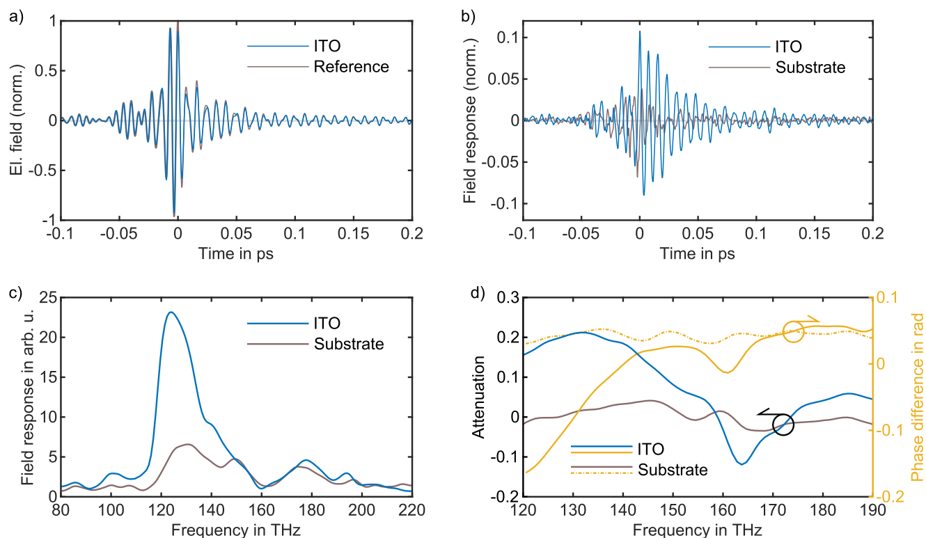
Figure 2. Transient electric field response and spectral characterization of the ITO nanocrystal thin film. a) Electric field of the transmitted excitation pulses from the ITO and substrate sample at the fluence of 75 \mu\text{J cm}^{-2} . The substrate measurements serve as reference measurements in this study. b) Calculated sample response obtained by subtracting the resolved electric field of the ITO from the reference at the same fluence (blue curve). Prior to subtraction, the two fields were temporally aligned by maximizing their cross-correlation within the window of -80 fs to -10 fs. The gray curve represents the averaged residual electric field from four consecutive reference measurements. c) Fourier transform of the ITO response, indicating the bandwidth of the response. The amplitude shows the magnitude of the attenuation in the ITO. d) The complex transmission spectrum of the sample, which is derived from the Fourier transformation of the transmitted electric field of ITO and the reference separately. The yellow curve indicates the spectral phase.
