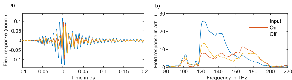
Figure 5. Damage threshold of the ITO nanocrystal thin film. a) Irreversibility of the optical switching at the fluence of 3.3 \text{ mJ cm}^{-2} . b) Spectral response of the switch at 3.3 \text{ mJ cm}^{-2} .
