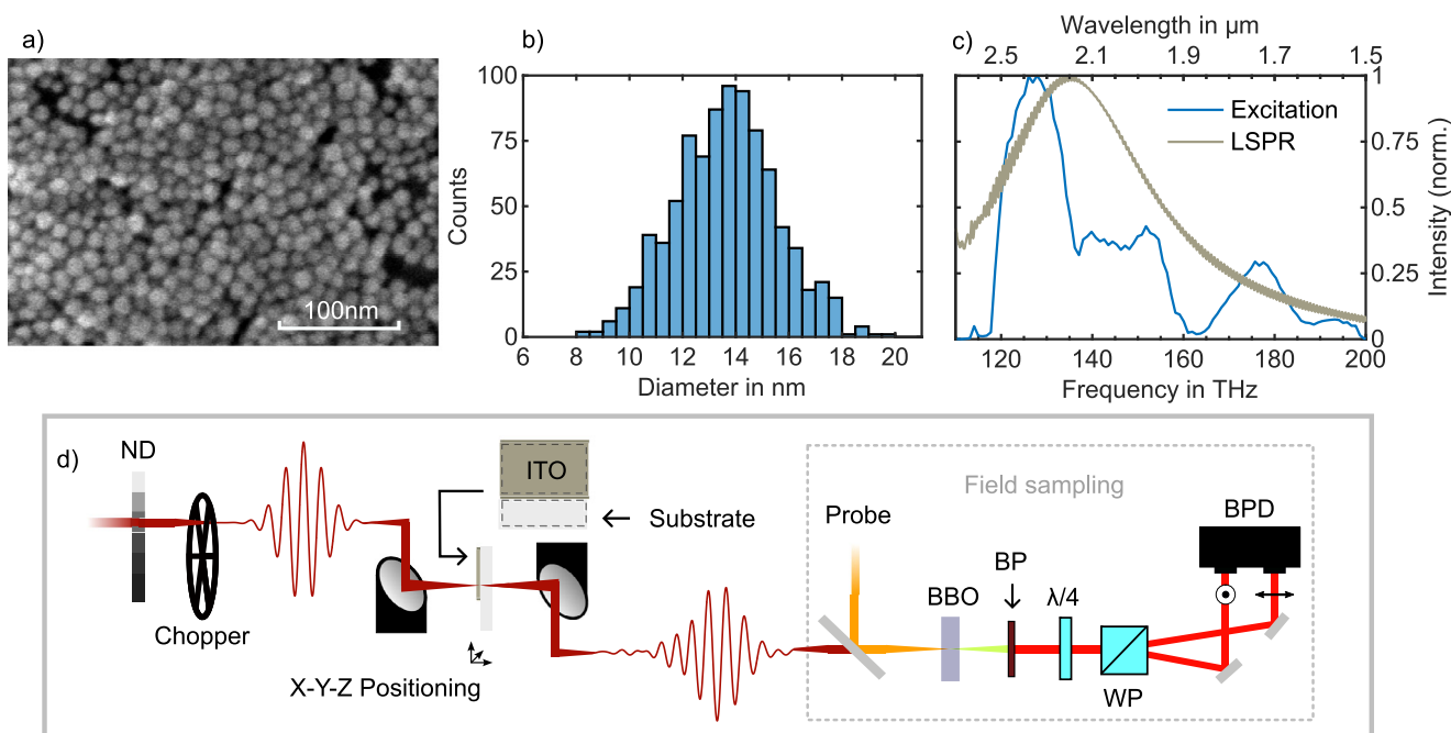
Figure 1. Structural, spectral, and experimental characterization of ITO nanocrystal thin films. a) Top-view scanning electron microscopy (SEM) micrograph of ITO nanocrystal. b) Statistical evaluation of the nanocrystals' diameter. In total, 871 crystals over an area of 470 nm×650 nm are analyzed, resulting in a mean nanocrystal diameter of 14 nm. c) Spectrum of the 10.7 fs excitation pulses (blue curve). The LSPR spectrum of the nanocrystals thin film (gray curve), measured by a wavelength scanning spectrometer. d) Schematic of the experiment. The sample consists of a borosilicate substrate with two areas of "ITO-coated" and "uncoated." The uncoated section serves as a reference for the measurement. The sample is positioned at the excitation beam focus, while the beam is modulated at 10 kHz by a mechanical chopper placed before the sample in the optical path. The fluence is varied from 10 \mu\text{J cm}^{-2} to 8 \text{mJ cm}^{-2} by adjusting both a variable neutral-density (ND) filter and the beam focus size. The transient field is resolved by employing fieldoscopy. ND: variable neutral density filter; BBO: beta barium borate; BP: bandpass filter; \lambda/4 : quarter wave plate; WP: Wollaston prism; BPD: balanced photo detector.
