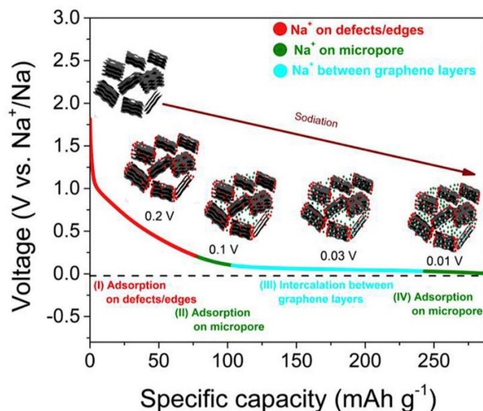
Figure 5: Sodiation mechanism in lignin derived BC. Reprinted with permission from ref. [150].
