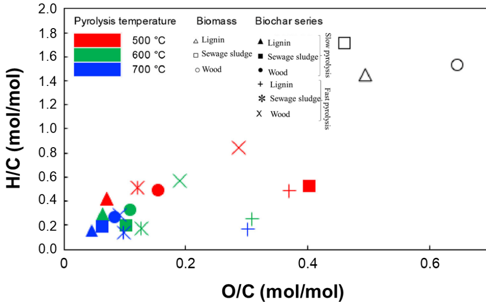
Figure 1: Van Krevelen diagram showing the effect of processing temperature on BC. Picture readapted and reprinted with permission (CC BY-NC-ND 4.0) from Bartoli et al. [35].
