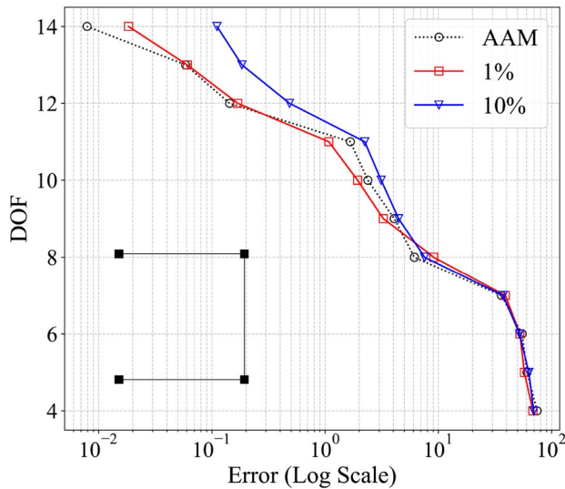
Fig. 14 BTD of the C beam not included in the network training. For each DOF level, curve report the minimum error achieved by the structural theories evaluated by FEM or NN
