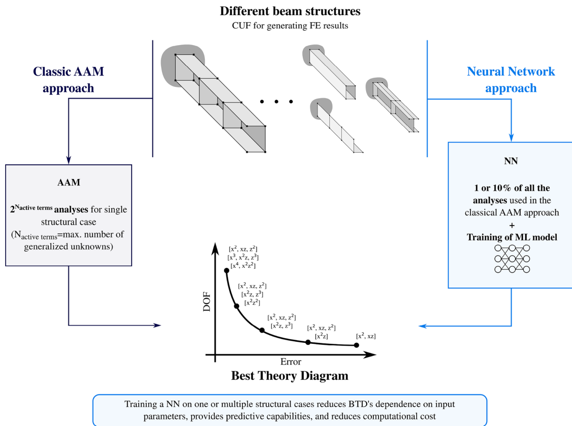
Fig. 3 AAM and DNN approach for developing BTD
