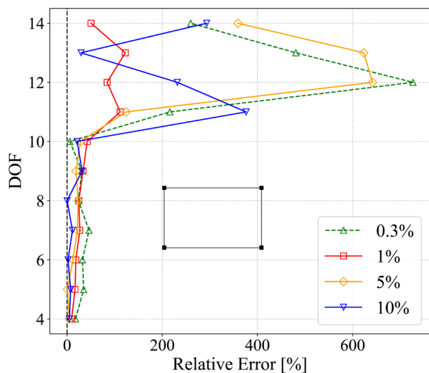
Fig. 11 Relative error of the BTD (in Fig. 10) between those derived from the DNN with different training dataset sizes and that derived from AAM for the Rectangular beam
