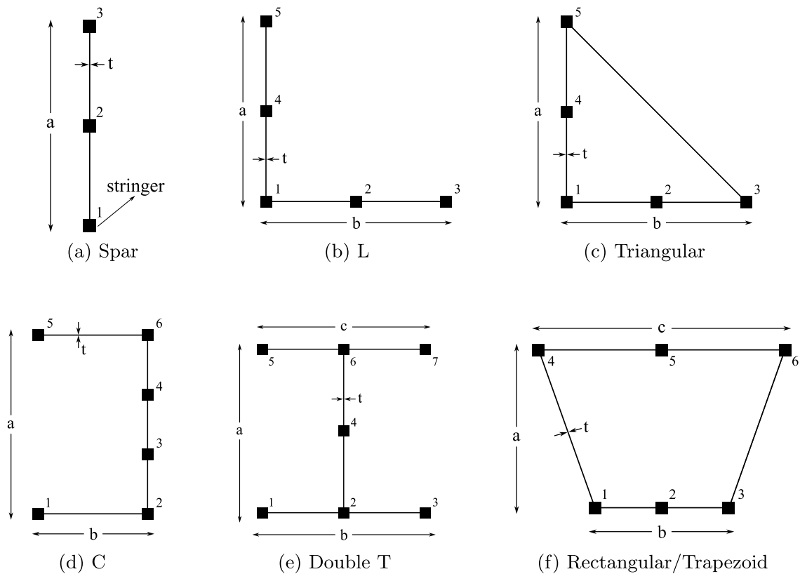
Fig. 7 Reference configurations for the 36 different cross-sections used for the network training
