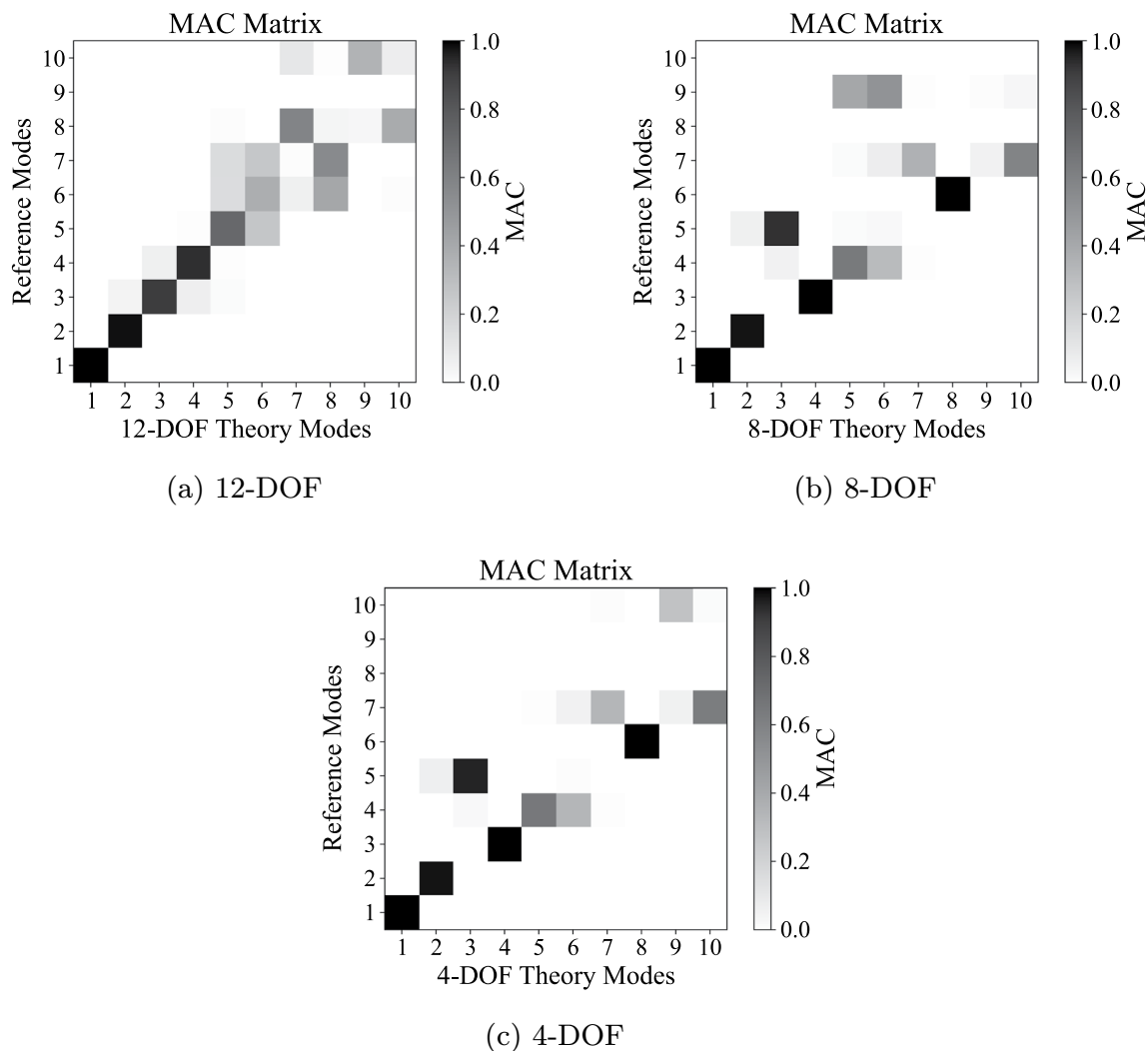
Fig. 16 MAC matrix for the Double T beam to quantify the matching of mode shapes obtained from the two structural theories, with values close to 1 indicating strong agreement between the modes
