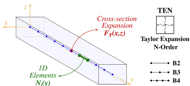
Fig. 1 Beam reference coordinate system
