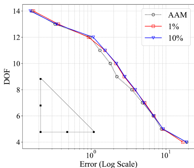
Fig. 12 BTM of the Triangular beam included in the network training. For each DOF level, curve report the minimum error achieved by the structural theories evaluated by FEM or NN
