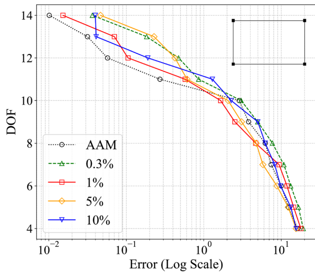
Fig. 10 BTD of the Rectangular beam from AAM and neural networks with different training dataset sizes. For each DOF level, curve report the minimum error achieved by the structural theories evaluated by FEM or NN
