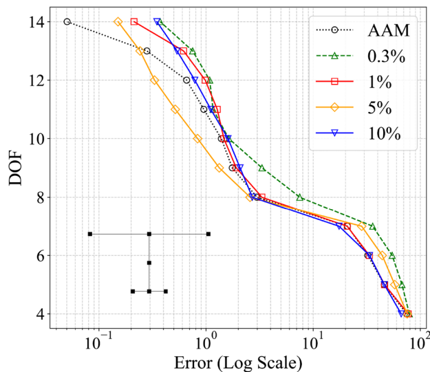
Fig. 8 BTD of the Double T beam from AAM, i.e., the FEM reference, and neural networks with different training dataset sizes—for each DOF level, curve report the minimum error achieved by the structural theories evaluated by FEM or NN
