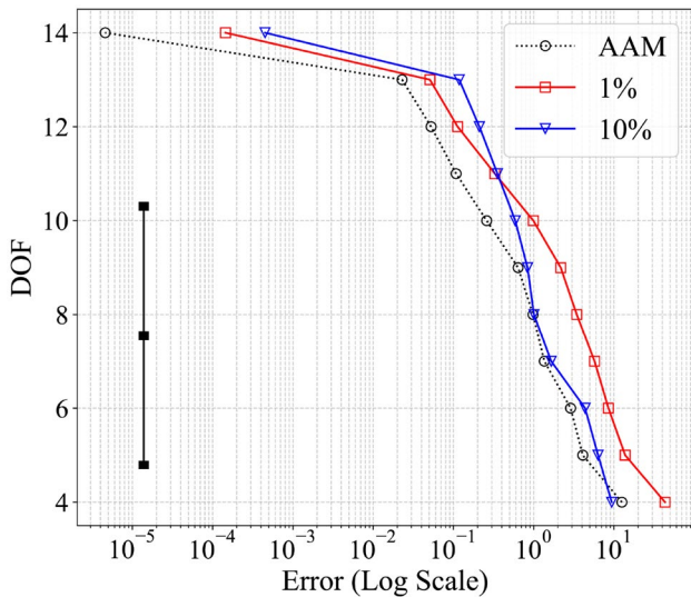
Fig. 15 BTD of the Spar beam not included in the network training. For each DOF level, curve report the minimum error achieved by the structural theories evaluated by FEM or NN
