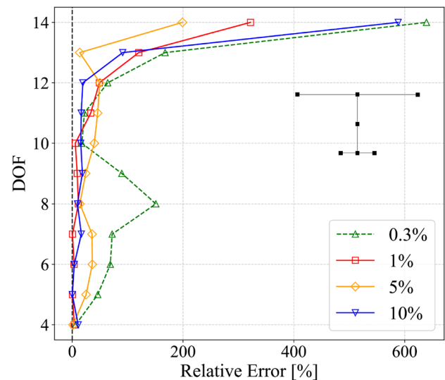
Fig. 9 Relative error of the BTD (in Fig. 8) between those derived from the DNN with different training dataset sizes and that derived from AAM for the Double T cross-section beam
