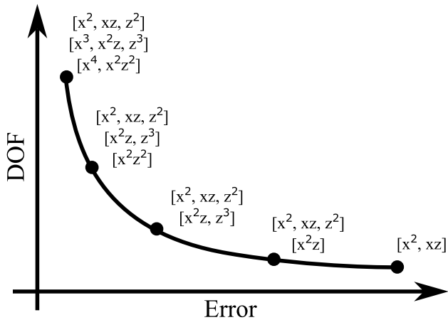
Fig. 2 A Best Theory Diagram (BTD) for 1D theories
