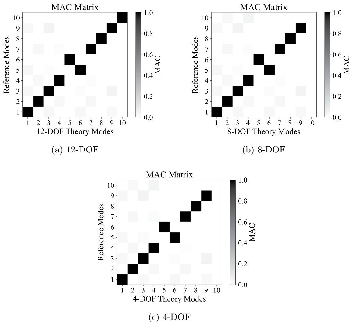
Fig. 17 MAC matrix for the Rectangular beam—It quantifies the correlation between mode shapes obtained from the two structural theories, with values close to 1 indicating strong agreement between the modes
