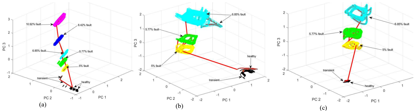
Fig. 5. The GCCA input quantization of IM SITF datasets - (a) No load, (b) 25% Load, (c) 40% Load
