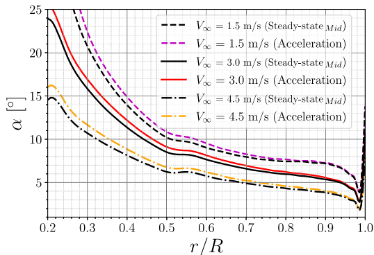
Fig. 15 Angle of attack \alpha distribution as a function of r/R extracted at midmaneuver for different V_\infty values.
