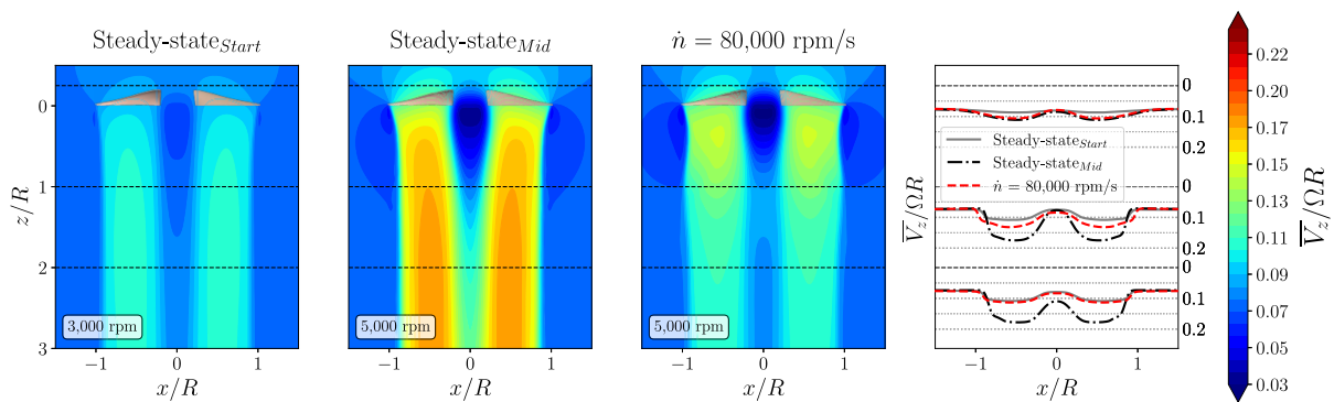
Fig. 13 Color maps of \bar{V}_z/\Omega R along with velocity profiles extracted at z/R = -0.25, 1 , and 2 (indicated by black dashed lines).
