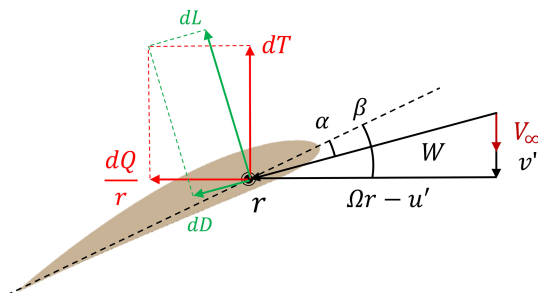
Fig. A1 Schematic representation of a blade element at a distance r from the propeller's hub.
