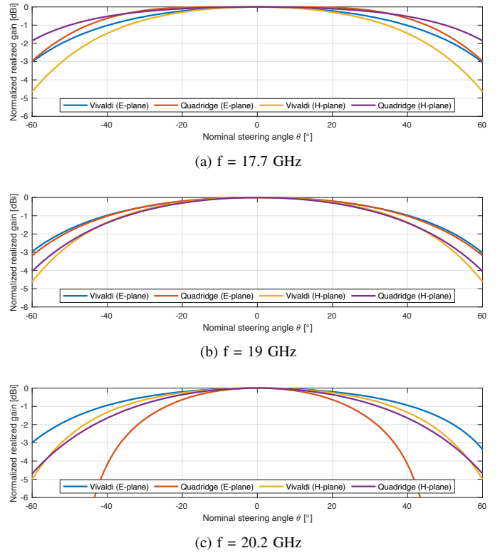
Fig. 3: AEP comparison between antennas at E and H planes
