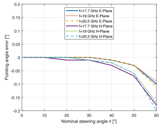
Fig. 7: Pointing error
