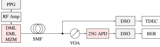
Fig. 1: Experimental setup
