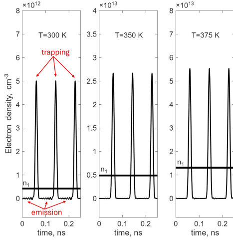
Fig. 6: Class A time domain electron density at high power ( P_{\text{out}} = 30 dBm) in the selected point in the drain depleted region. Thick solid lines show the n_1 value ( T -dependent).
