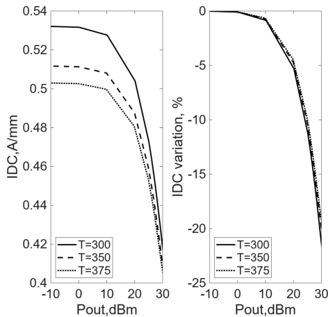
Fig. 4: Class A DC component of the LS drain current with increasing output power at the three analyzed temperatures.
