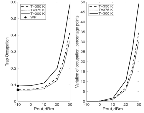
Fig. 7: Class A trap occupation vs. output power for the selected point in the drain depleted region.
