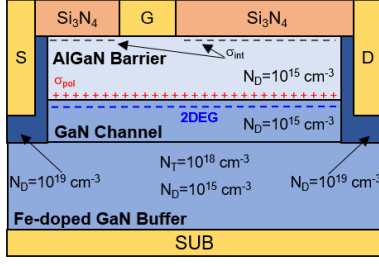
Fig. 2: Cross section of the simulated device. The gate length is 150 nm.
