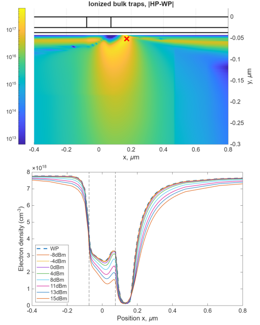
Fig. 5: Class A DC behavior. Top: difference of occupied traps DC component at available input power P_{av} = 15 dBm (HP) and at the DC working point (WP). The “x” represents the point investigated in Figs. 6-7. Bottom: cross section of the electron density in the channel, 1 nm below the AlGaIn/GaN interface, as a function of the available power.
