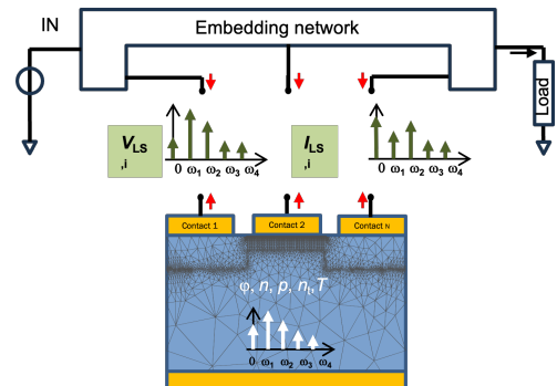
Fig. 1: Schematic representation of the software set-up for mixed-mode HB TCAD analysis. The external embedding circuit includes microwave components as ideal idlers, bias tees and harmonic tuned terminations.
