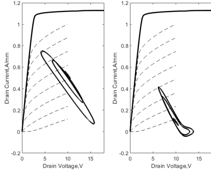
Fig. 3: DLL on the output characteristic for several input available powers: P_{av} = -25 dBm (almost invisible), -5 dBm, 10 dBm and 15 dBm. Left: class A bias point. Right: class AB bias point.
