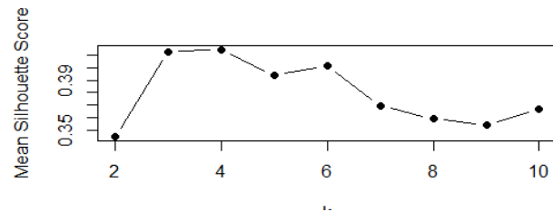
Fig. 9: Value of the optimal number of clusters for hierarchical clustering
