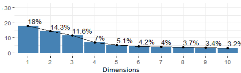
Fig. 7: Distribution of Explained Variance across the First Ten Principal Components
