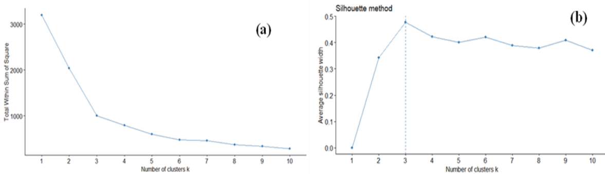
Fig. 11: Optimal number of clusters with (a) the Elbow method; (b) average silhouette method
