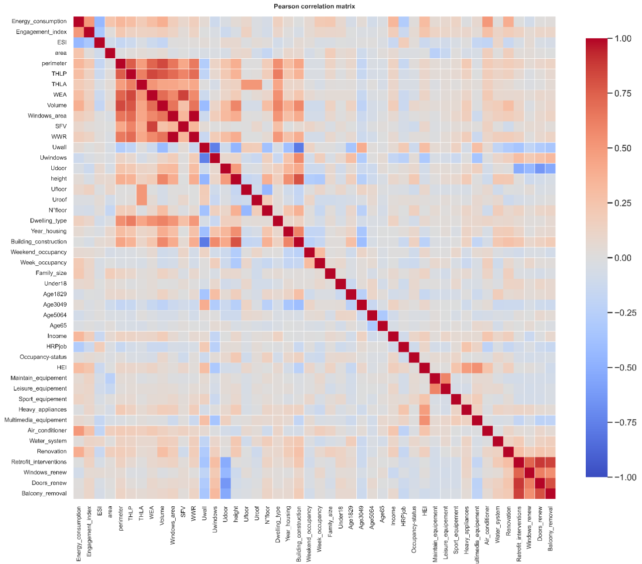
Fig. 6: Pearson Correlation matrix
