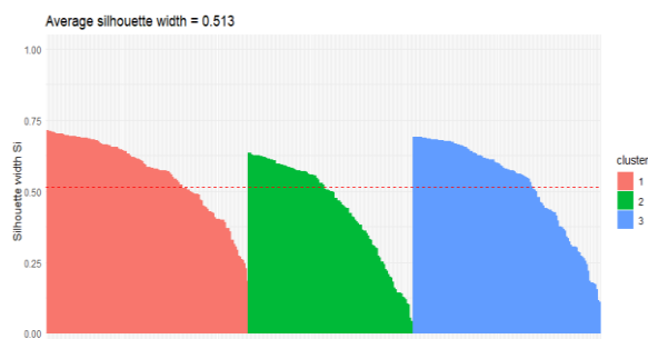
Fig. 15: average silhouette width of K-means clustering
