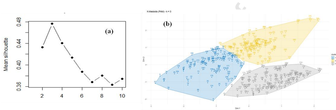
Fig. 13: (a) search for optimal k number with K-medoid clustering, (b) K-medoid clustering results.
