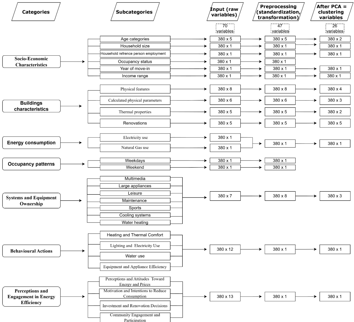
Fig. 8: Workflow of Variable Transformation and Dimensionality Reduction Across Data Processing
