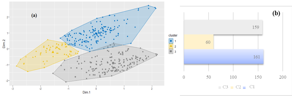
Fig. 10: Hierarchical clustering plot results; (a) clusters visualisation , (b) observations distribution in the clusters
