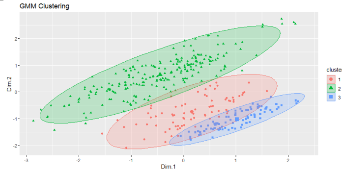
Fig. 14: GMM clustering results
