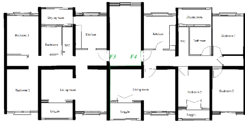
Type 01: 5-story multi-family residential buildings with 2 dwelling units per floor, built using brick masonry construction (1970-1995)
