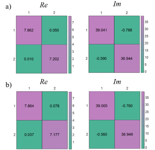
Fig. 10. Antenna input impedance: a) Old FELICE b) New FELICE.
