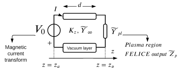
Fig. 1. Equivalent circuit representation. In this model, the magnetic current \widetilde{M}_a passes over into a lumped voltage source, the vacuum region is modeled as a transmission line of length d , and the plasma response is encapsulated in the admittance \widetilde{Y}_{pl} , which corresponds to the inverse of the plasma 2 \times 2 impedance matrix computed by the FELICE code.
