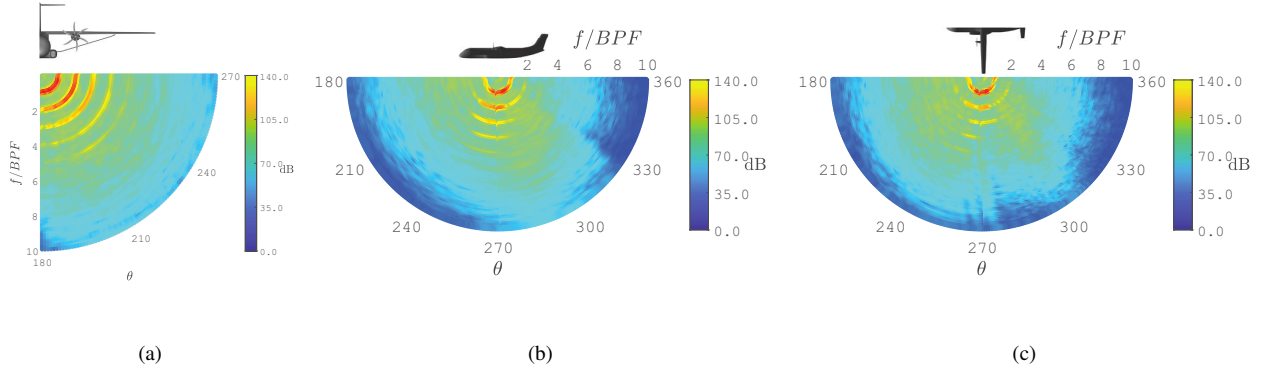
Fig. 6 Frequency spectra directivity plot in the frontal plane (a), lateral plane (b) and top plane (c). The frequency is scaled by the Blade Passing Frequency (BPF).
