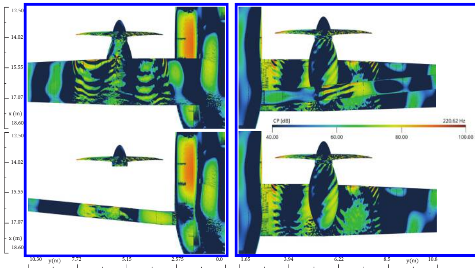
Fig. 10 Surface acoustic pressure distribution contributing to far-field Noise at frequency band centered at 2 times the BPF, visualized using Dassault Systems optydb_pfnnoisescan software. The top-left image depicts the wing's upper side distribution, while the bottom-left image reveals the upper side of the strut and fuselage sponson by hiding the wing and nacelle. On the top-right, the lower side of the strut is illustrated, whereas the bottom-right image displays the wing's underside by hiding the strut surface.
