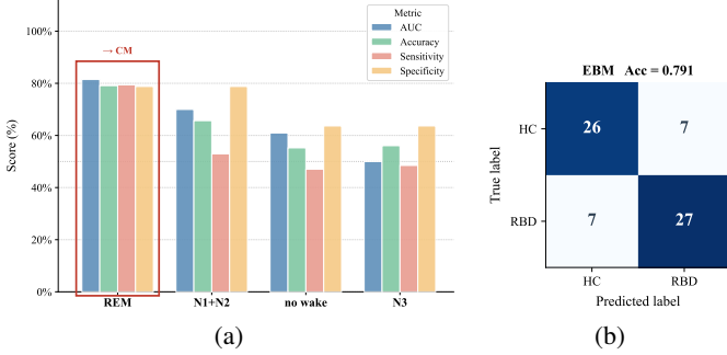
Fig. 2. (a) Classification performance (AUC, accuracy, sensitivity, specificity) across sleep stages. (b) Confusion matrix for the REM stage.
