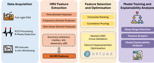
Fig. 1. Overview of the proposed HRV-based iRBD detection pipeline.
