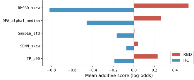
Fig. 5. Mean additive EBM score as log-odds per class in REM stage.
