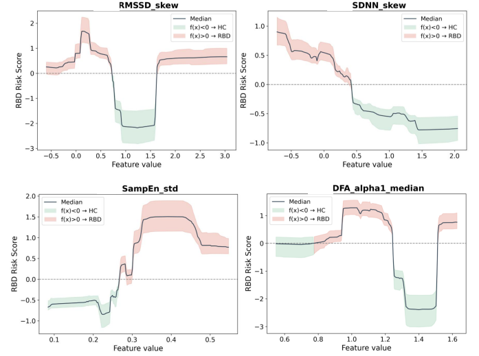
Fig. 6. EBM shape functions for the four most stable features (REM stage). Solid line: median f_j(x_j) across LOSO folds; shaded band: interquartile range. Green: f_j < 0 (toward HC); red: f_j > 0 (toward iRBD).
