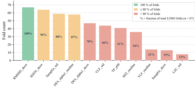
Fig. 3. Feature selection stability across LOSO folds. Each bar indicates in how many of the N folds a given feature was included in the final model.
