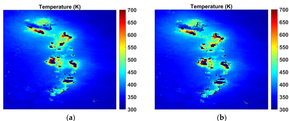
Figure 3. Temperature fields were estimated using (a) SISSI simulated channels; and (b) SISSI-like channels reconstructed by applying the CS algorithm on simulated CS acquisition with CR = 50%.
