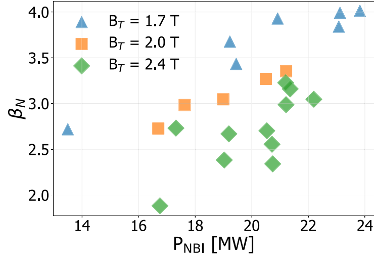
Figure 7. Maximum normalized beta \beta_N as a function of NBI heating power P_{\text{NBI}} (MW) for different toroidal magnetic fields.
