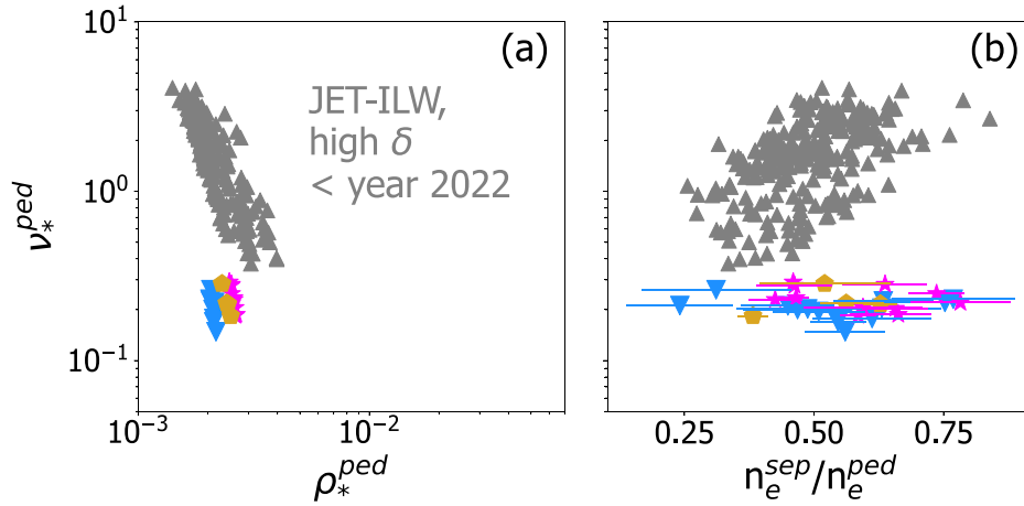
Figure 12. Ranges of pedestal collisionality as a function of normalized ion Larmor radius at the pedestal \rho_{i*}^{*,ped} (a) and as a function of separatrix density normalized to pedestal density (b). In color the explored parameter space with respect to earlier high-delta cases, depicted in gray. Colors in the new dataset indicate different isotope compositions: Deuterium (blue points), D–T (gold) and T-rich (magenta).
