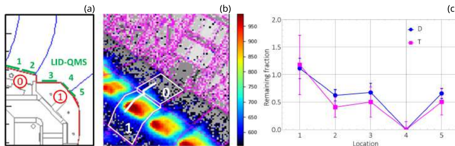
Figure 19. Change in fuel retention at the JET inner divertor following the Raised Inner Strike Point (RISP) plasma configuration. (a) Location of the poloidal LID-QMS scans (green numbers from 1 to 5). Inner strike point location for the RISP configuration is shown at the upper end of location 5 where the highest heat flux is expected (see [119] for details on RISP). (b) Infrared view during RISP operation, showing the most heated areas on tile 1 (reproduced from [56]). (c) remaining fraction of D and T after RISP cleaning at the locations shown in (a), calculated as the ratio between LID-QMS measurements before and after RISP. Post RISP measurements of D/T at location 4 are below the detection limit of LID-QMS (LID-QMS data taken from [123]). (b) Reproduced from [119]. The Author(s). CC BY 4.0.
