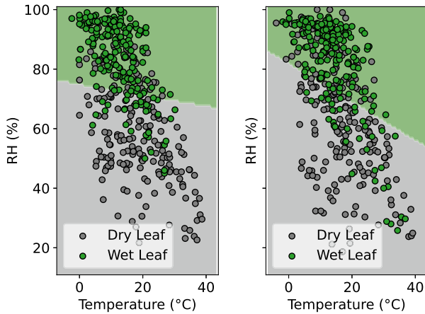
Fig. 5. Decision boundary for the LDA classifier in the temperature and RH domain, for the top leaf side (left), and bottom leaf side (right) using a leaf wetness threshold rule of 20%.
