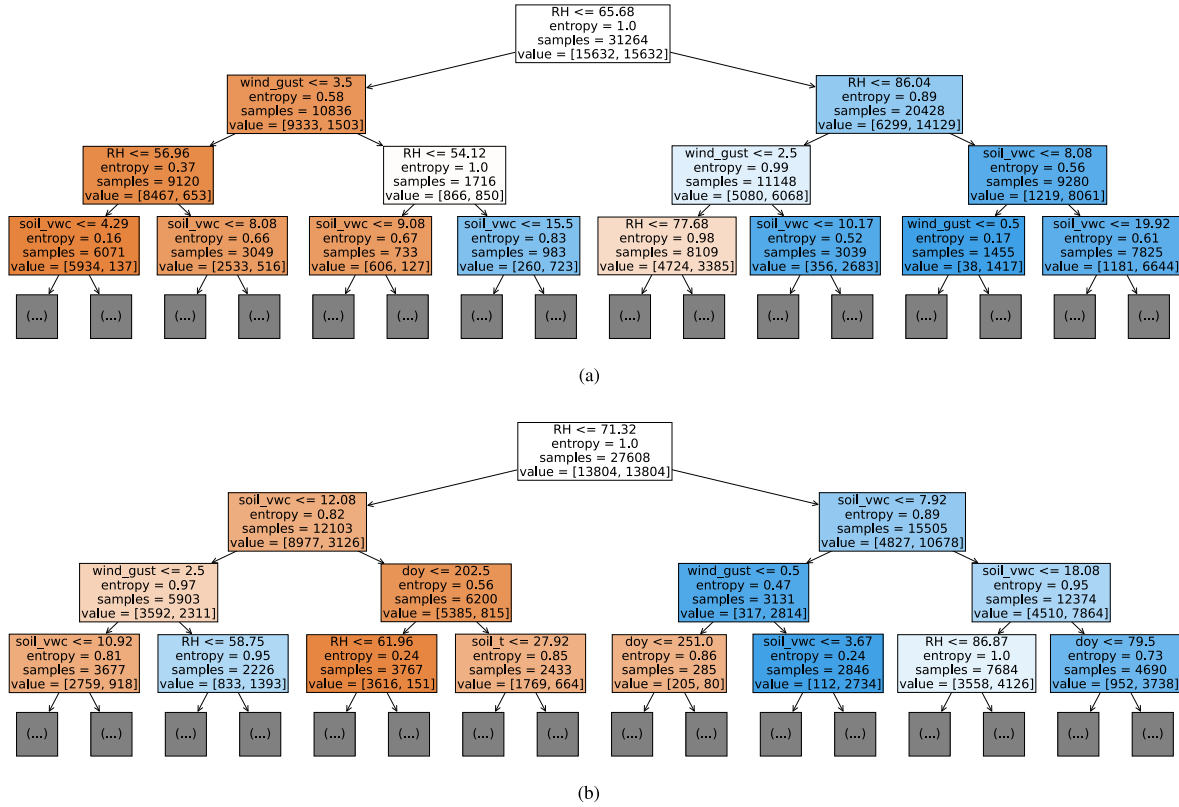
Fig. 6. First three levels of the DTs for both leaf sides, orange nodes are composed mainly of dry samples; blue ones are composed mainly of wet samples. (a) Top side. (b) Bottom side.
