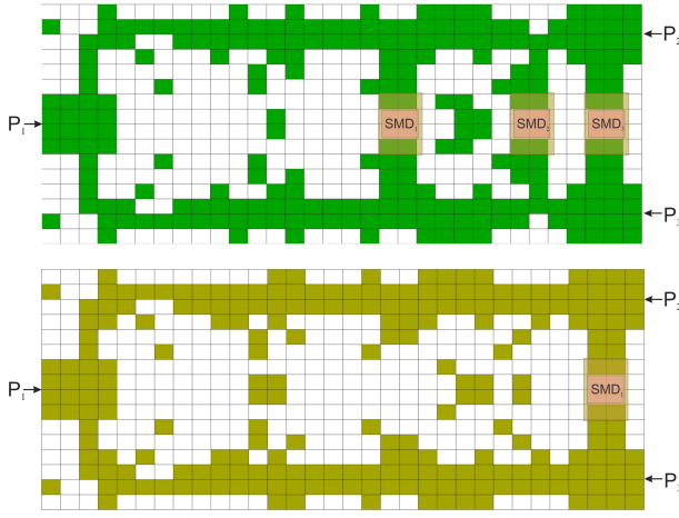
Fig. 2. Examples of pixelated layouts hosting three or one SMDs.
