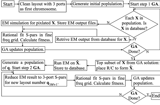
Fig. 1. Flowchart of the proposed 2-step genetic optimization for the design of microwave circuits with pixelated layout and lumped elements.
