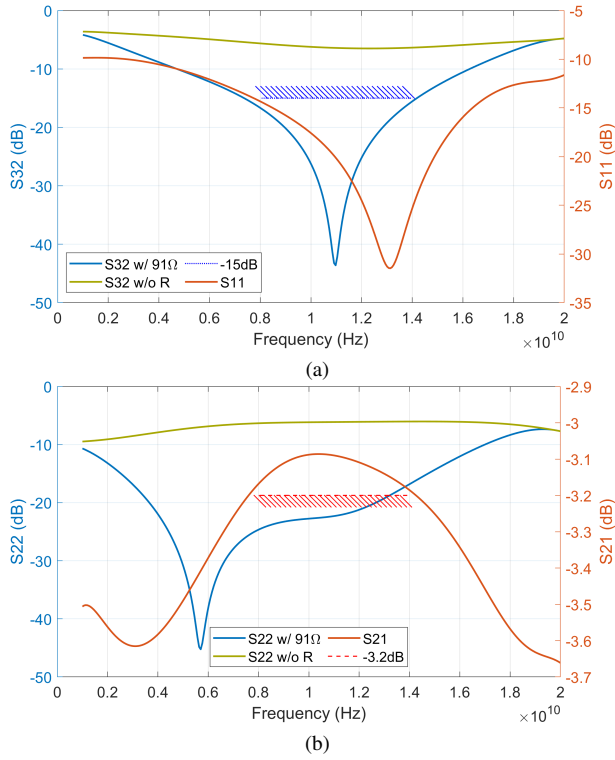
Fig. 3. Performance of the best pixelated layout with and without the SMD resistor: (a) input matching and isolation (-15 dB target); (b) output matching and transmission (-3.2 dB target).
