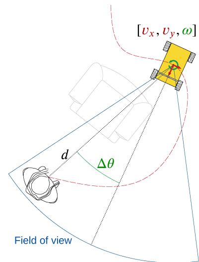
Fig. 1: Our person following solution exploits DWA planner to control linear velocities [v_x, v_y] while the DRL agent controls the angular velocity \omega to minimize the angle \Delta\theta and maintain the user within the camera's field of view. This approach allows the rover to keep monitoring the person while avoiding obstacles on a safe trajectory.
