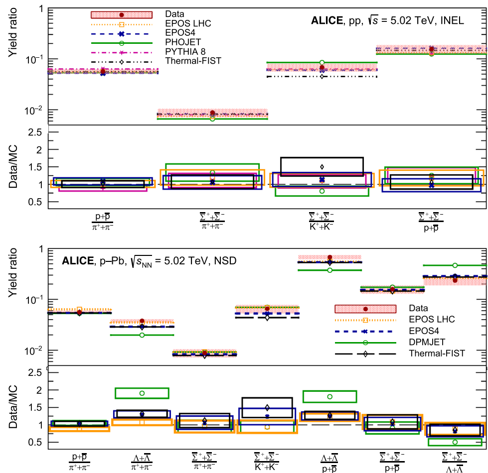
Fig. 10 Comparison of ratios of integrated yields of different particle species as shown in Table 4 ( \Sigma^- and \Sigma^+ yields are combined). Ratios are compared to predictions of EPOS LHC and EPOS4 [37,38], PHOJET and DPMJET [39], PYTHIA 8 [29], and Thermal-FIST [43] models
