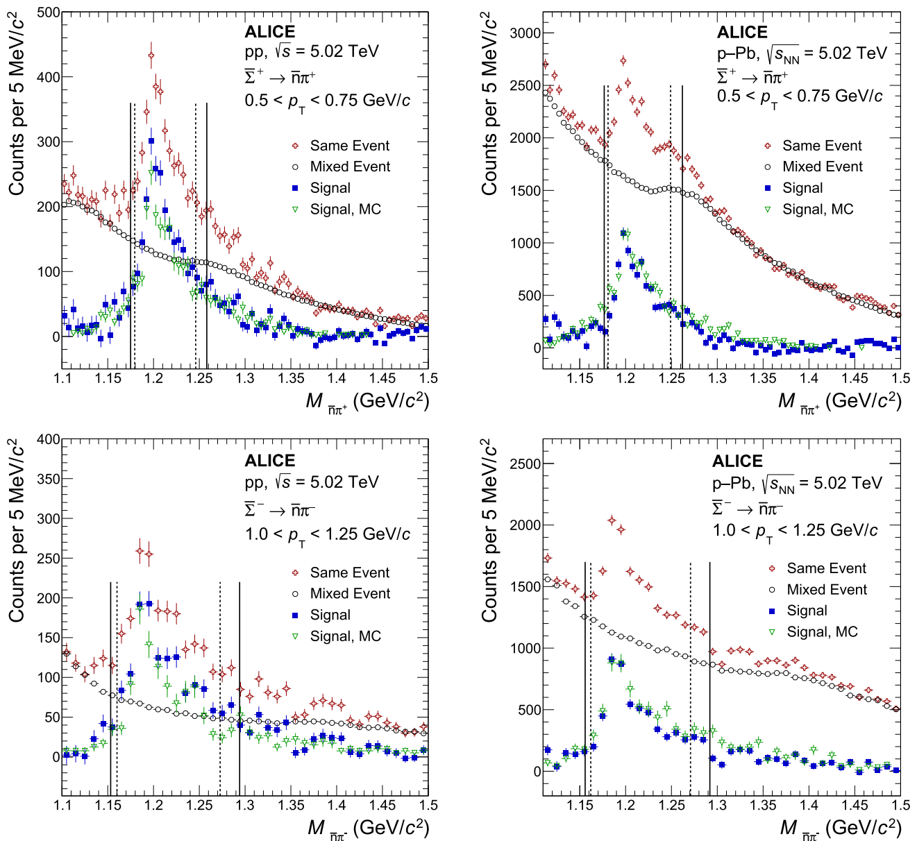
Fig. 4 Same event, mixed event, signal from data, and MC true signal invariant mass distributions of \bar{n}\pi^+ (top row) and \bar{n}\pi^- (bottom row) pairs in pp (left column) and p–Pb (right column) collisions for two selected p_T bins. Solid and dashed vertical lines represent integration
