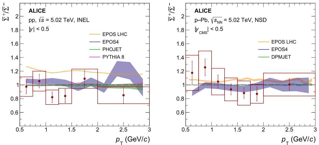
Fig. 8 Ratio of \Sigma^+ to \Sigma^- spectra in pp and p–Pb collisions compared to predictions of EPOS LHC and EPOS4 [37,38], PYTHIA 8 [29], PHOJET and DPMJET [39] models
