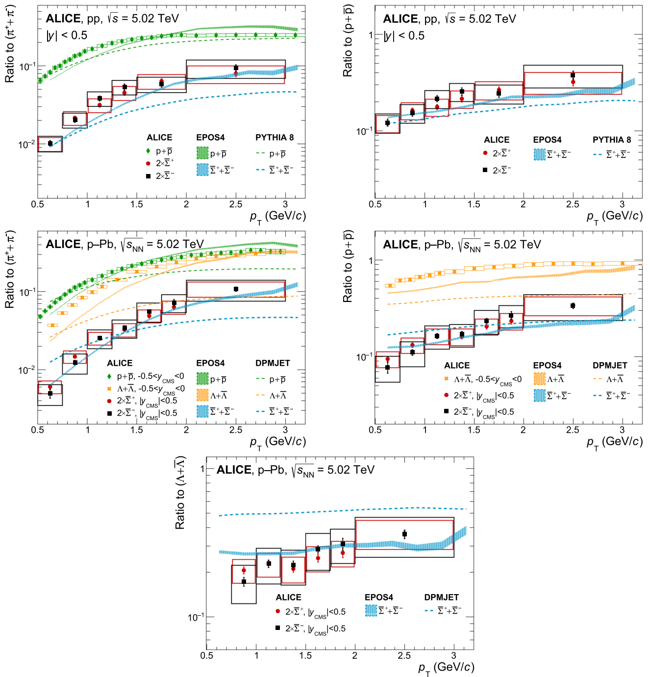
Fig. 9 p_T -differential ratios of \bar{\Sigma}^- , \bar{\Sigma}^+ , \Lambda and protons to pions, protons, and \Lambda (in the case of p-Pb collisions) in pp (top row) and p-Pb (middle and bottom rows) collisions. In the ratios for p-Pb col-
