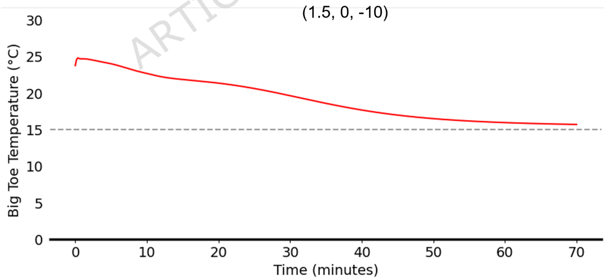
Figure 9. LSTM prediction under stillness with the same insulation as in Figure 8, but at an ambient temperature of -10^{\circ}\text{C} . The predicted curve does not reach the safety threshold within the observation window.
