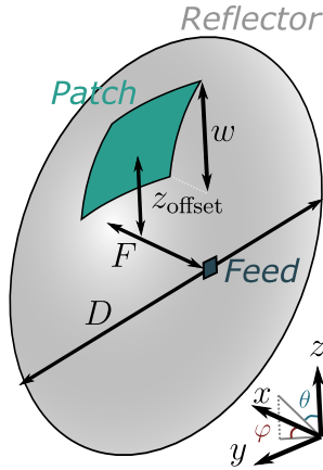
Fig. 2. Geometry of the antenna.
