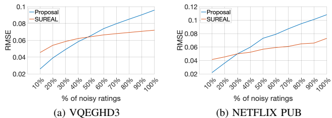
Fig. 5. Robustness of the approaches to synthetic noise added to the ratings of 10% of subjects in each dataset while disregarding the fact that subject are less inconsistent at the extreme of the quality scale. The experiment is repeated with 100 different seeds and the average RMSE is reported.
